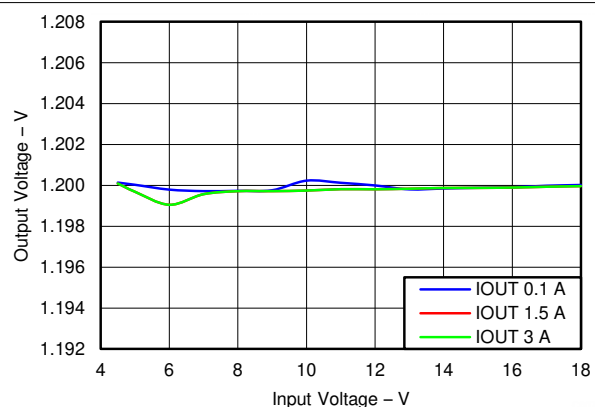
Figure 6-6. Buck1, Line Regulation
