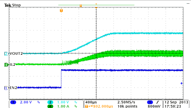
Figure 9-5. BUCK2, Soft-Start With Full Load
