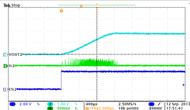
Figure 9-4. BUCK2, Soft-Start With No Load
