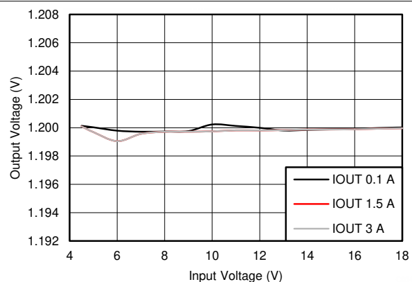
Figure 7-6. BUCK1, Line Regulation
