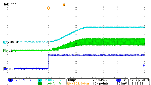
Figure 9-7. BUCK3, Soft-Start With Full Load
