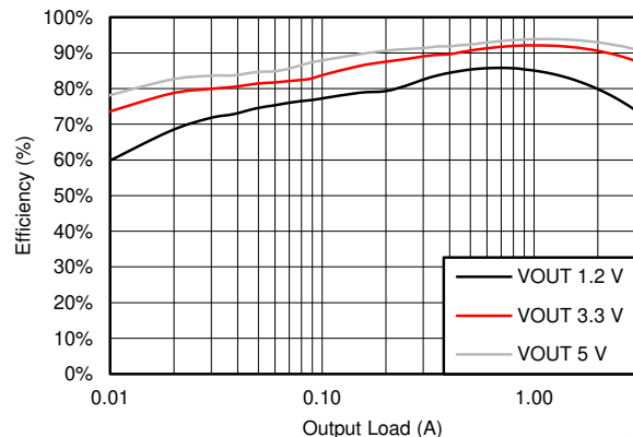
Figure 7-1. BUCK1 Efficiency
