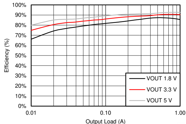
Figure 7-2. BUCK2 Efficiency
