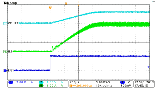
Figure 9-3. BUCK1, Soft-Start With Full Load
