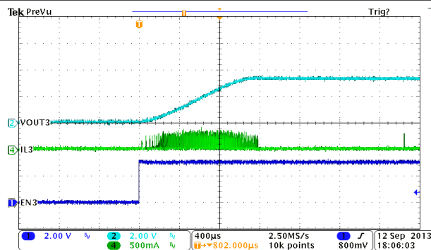
Figure 9-6. BUCK3, Soft-Start With No Load
