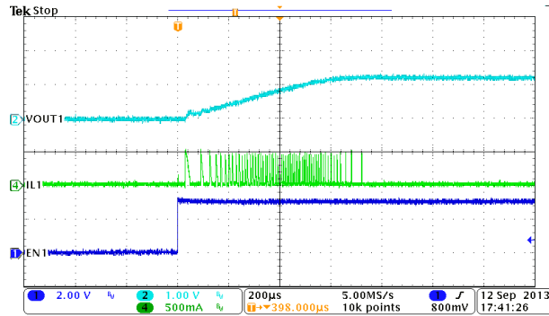
Figure 9-2. BUCK1, Soft-Start With No Load
