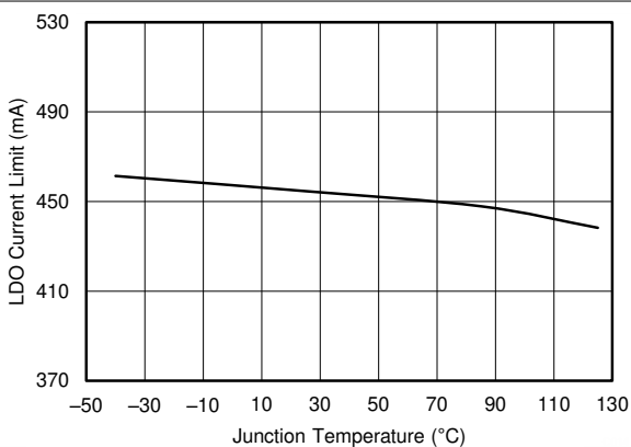
Figure 7-23. LDO Current Limit vs Temperature
