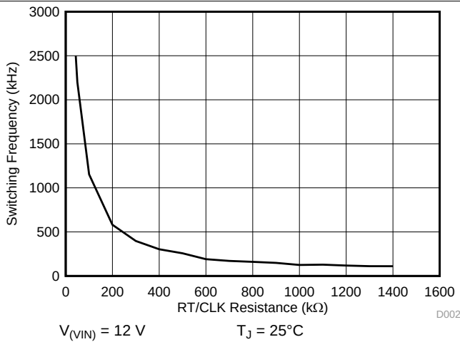
Figure 3. Buck-Regulator Switching Frequency vs RT_CLK Resistance
