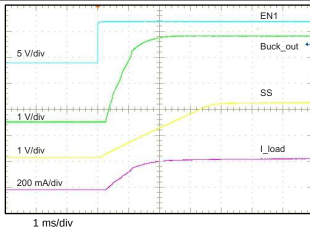
Figure 24. Buck-Regulator Startup Operation
