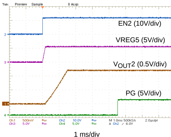
Figure 33. VOUT2 = 1.2V Soft-Start IOUT2 = 2.5A
