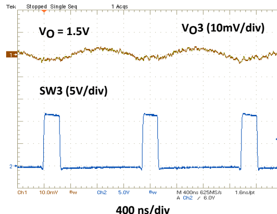
Figure 27. VOUT3 = 1.2V, Ripple Voltage at IOUT1 = 1.5A
