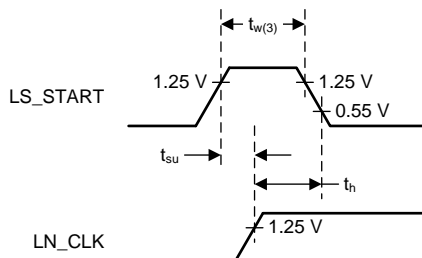
Figure 2. LS_START Timing Requirements
