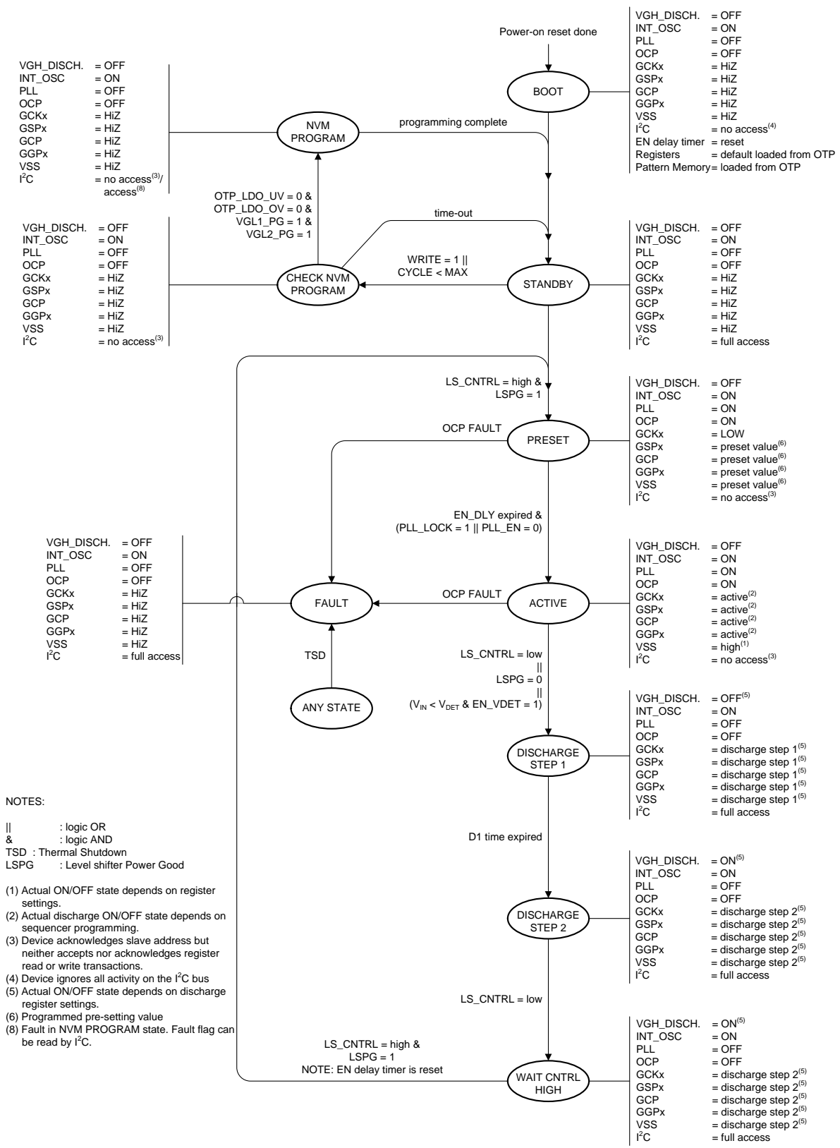
Figure 22. Functional State Diagram
