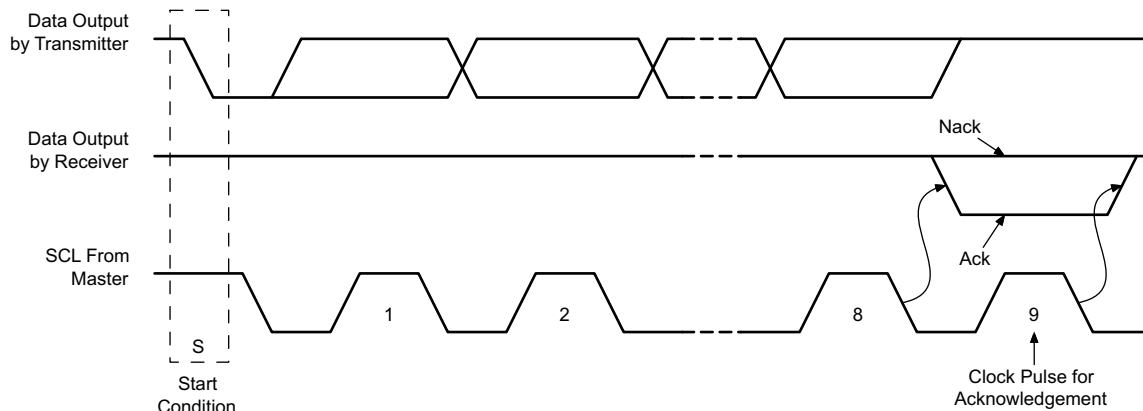
Figure 8-25. I²C Acknowledgment
