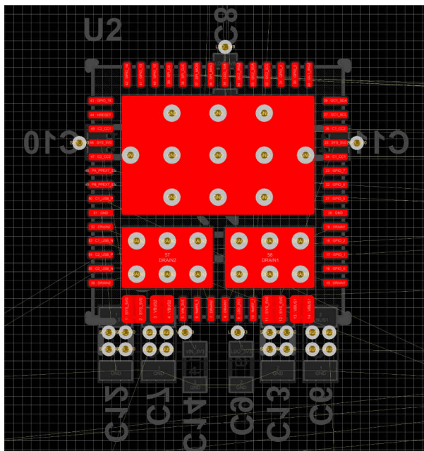
Figure 11-10. System Capacitors Placement Top Layer
