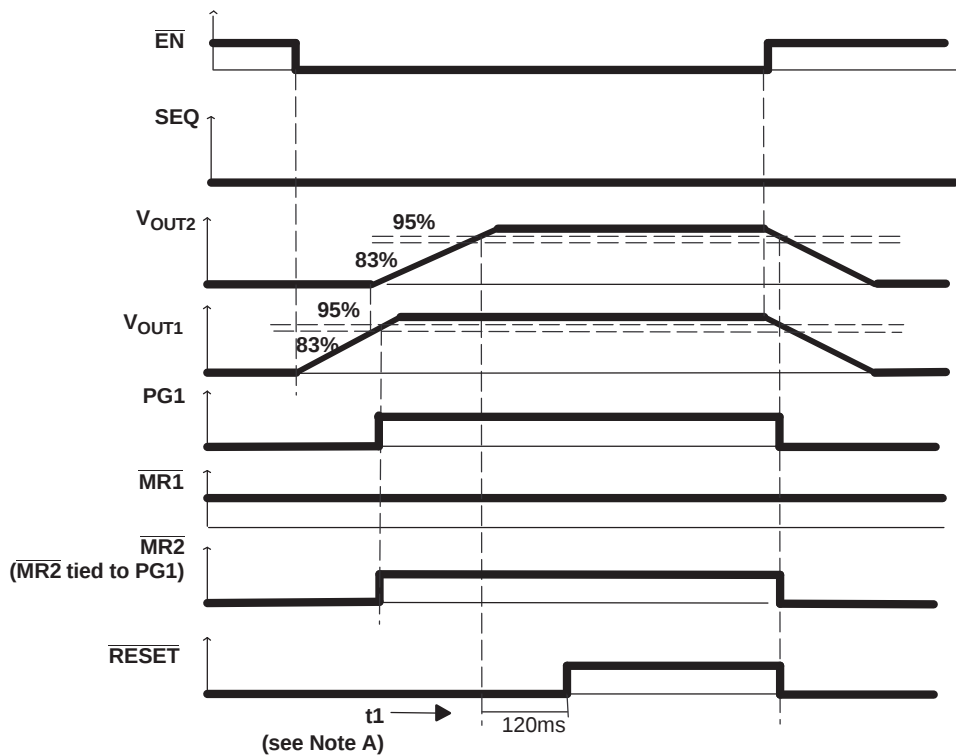
Figure 40. Timing when \overline{\text{SEQ}} = Low
