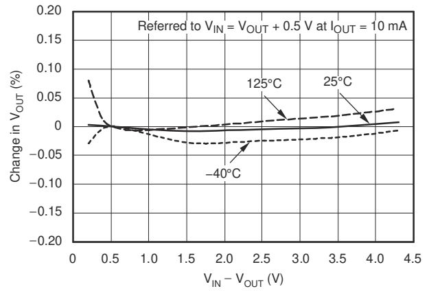
Figure 5-2. Line Regulation
