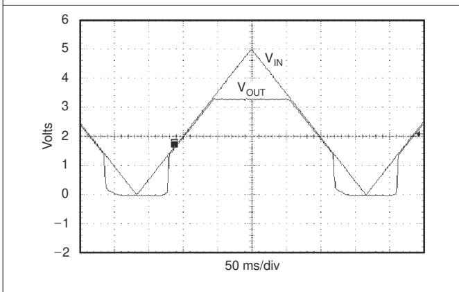
Figure 5-21. TPS73633 Turn-On Response
