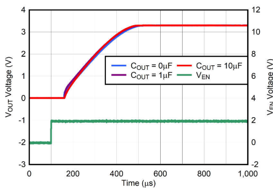
Figure 5-33. TPS73701 Turn-On Response
