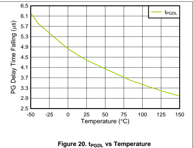
Figure 20. t_{PGDL} vs Temperature
