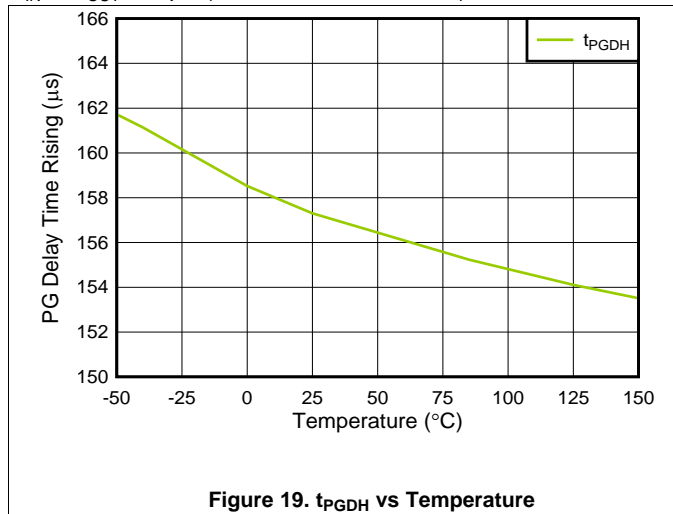
Figure 19. t_{PGDH} vs Temperature
