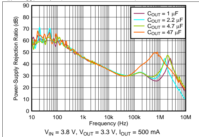
Figure 37. PSRR vs Frequency and C_{OUT}
