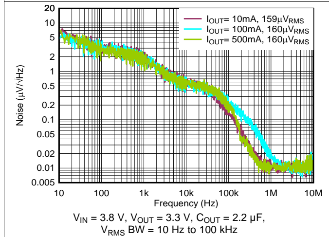
Figure 41. Output Spectral Noise Density
