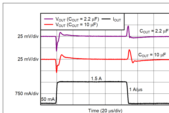
Figure 7-2. Load Transient Response
