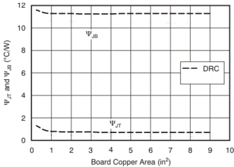
Figure 7-5. \Psi_{JT} and \Psi_{JB} vs Board Size
