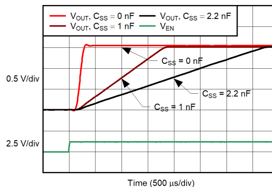
Figure 7-3. Turn-On Response
