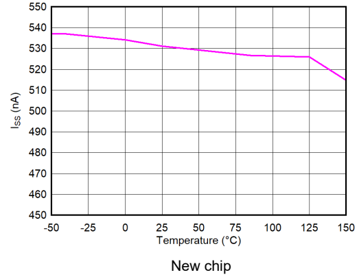
Figure 5-26. Soft-Start Charging Current ( I_{SS} ) vs Temperature ( T_J )
