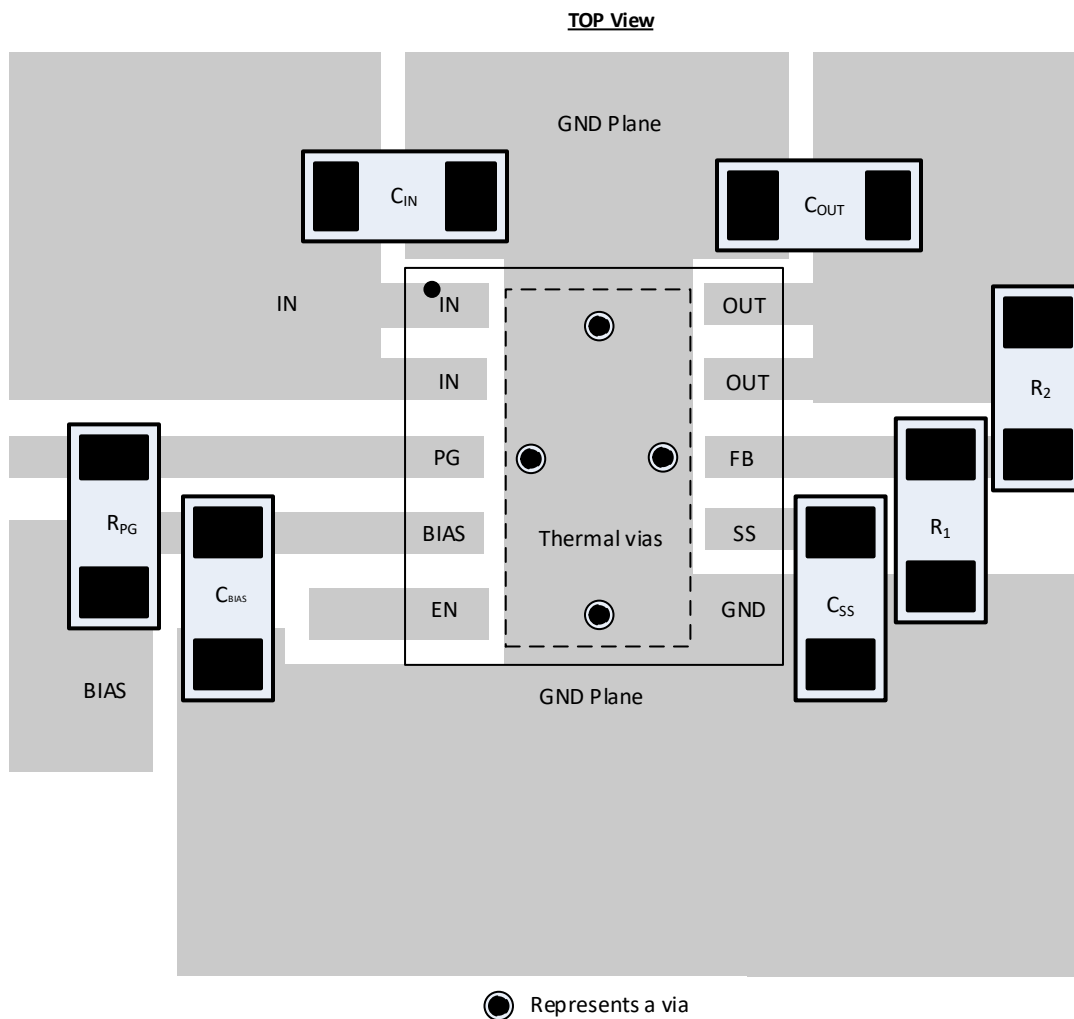
Figure 7-4. Example Layout
