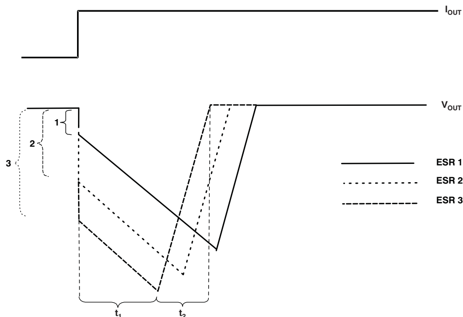
Figure 24. Correlation of Different ESRs and Their Influence to the Regulation of V_{OUT} at a Load Step From Low-to-High Output Current
