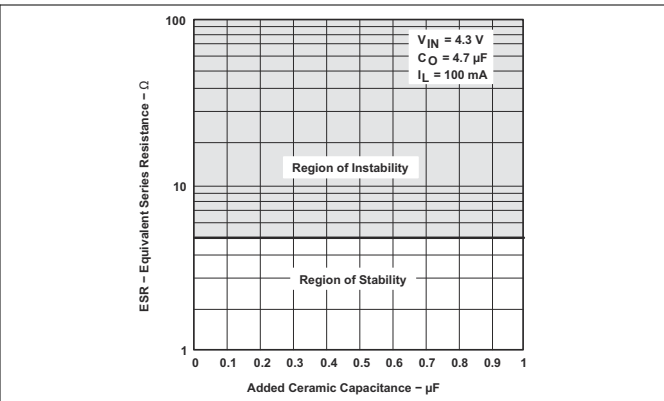
Figure 5-47. TPS76933 Typical Regions of Stability ESR vs Added Ceramic Capacitance (Legacy Chip)
