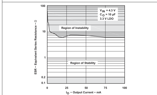
Figure 5-46. TPS76933 Typical Regions of Stability ESR vs Output Current (Legacy Chip)
