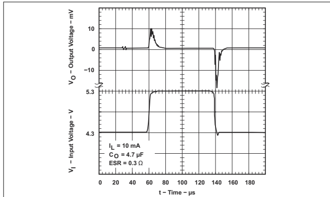
Figure 7-10. TPS76933 Line Transient Response (Legacy Chip)
