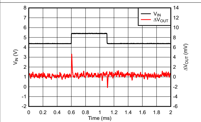
Figure 7-7. TPS77015 Line Transient Response (Legacy Chip)
