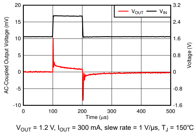
Figure 6-34. Line Transient
