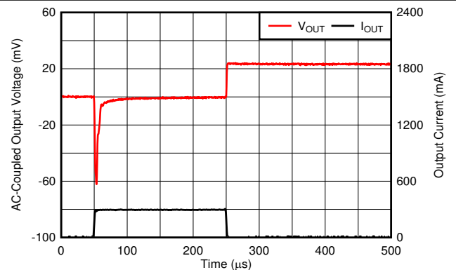
Figure 6-50. Load Transient
