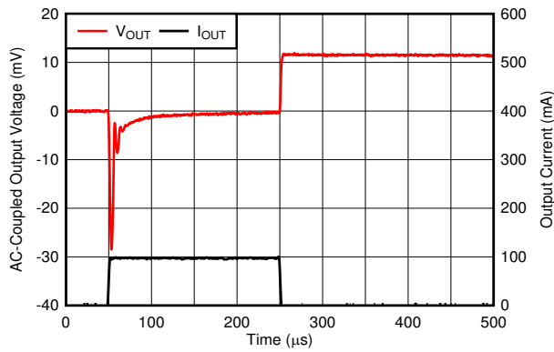
Figure 6-49. Load Transient
