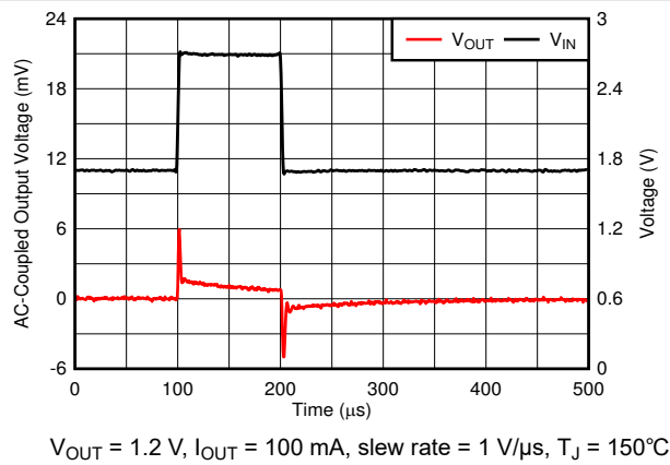
Figure 6-31. Line Transient
