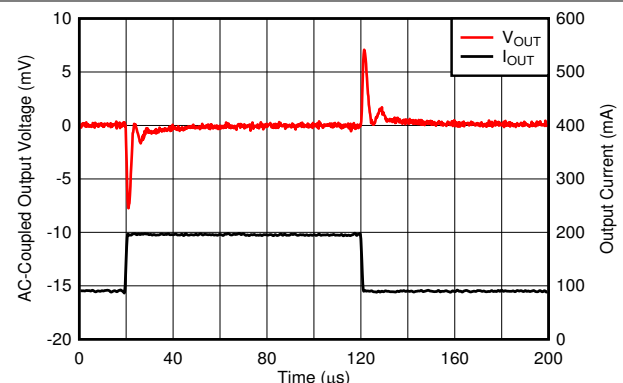
Figure 6-52. Load Transient
