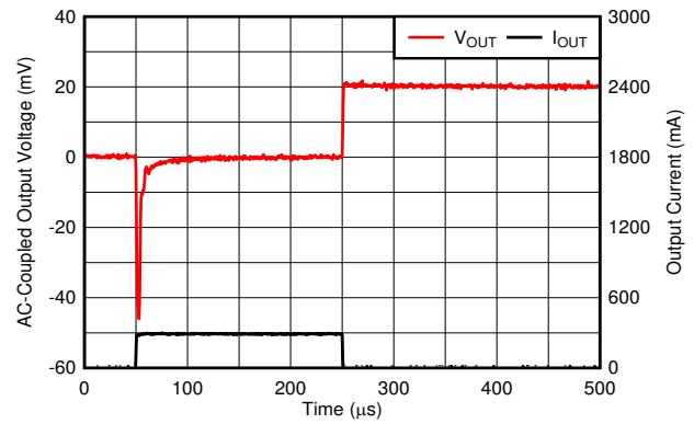
Figure 6-50. Load Transient
