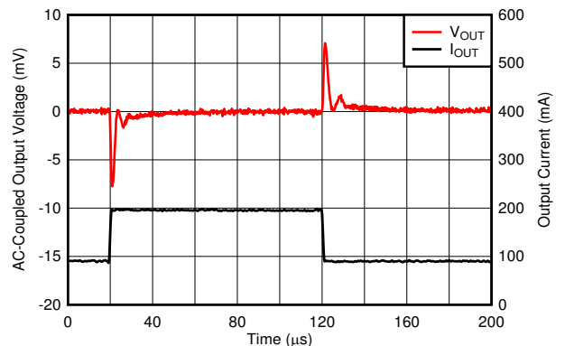
Figure 6-52. Load Transient
