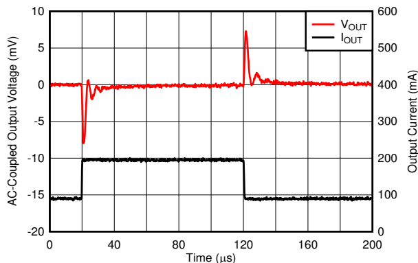
Figure 6-51. Load Transient
