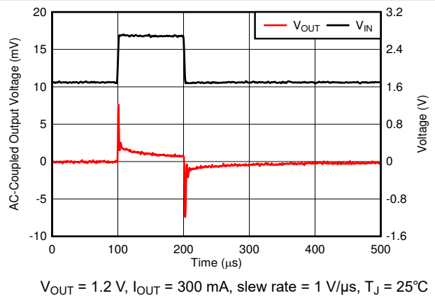
Figure 6-32. Line Transient
