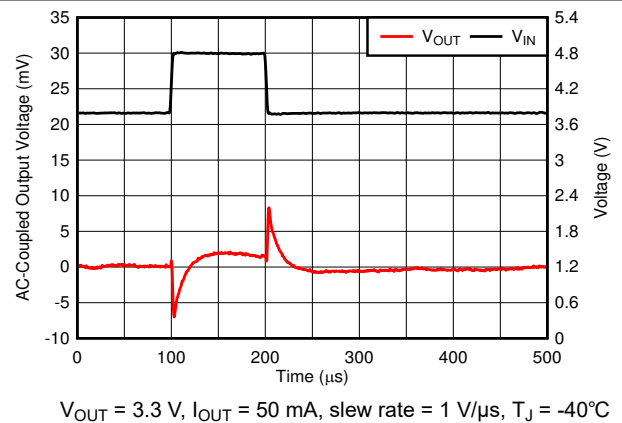
Figure 6-36. Line Transient
