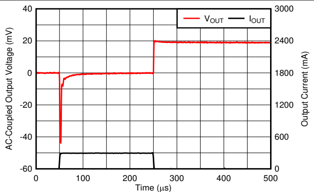
Figure 6-49. Load Transient
