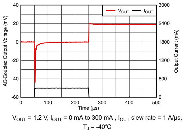
Figure 6-51. Load Transient
