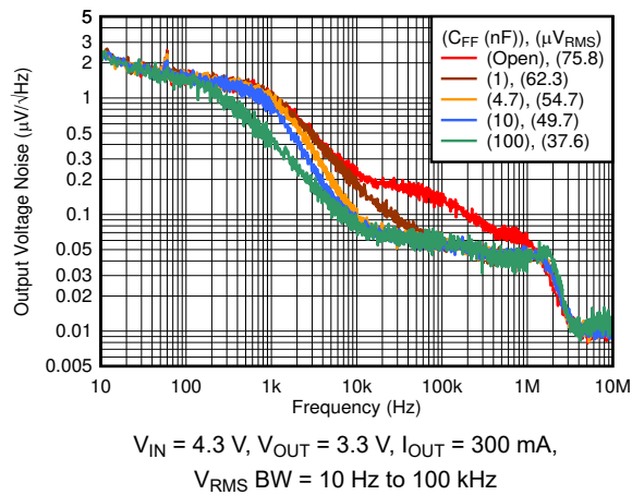
Figure 6-73. Output Noise vs Frequency and C_{FF}
