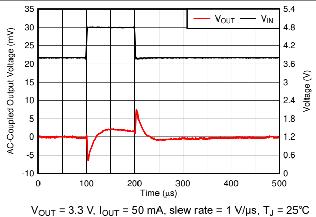
Figure 6-35. Line Transient
