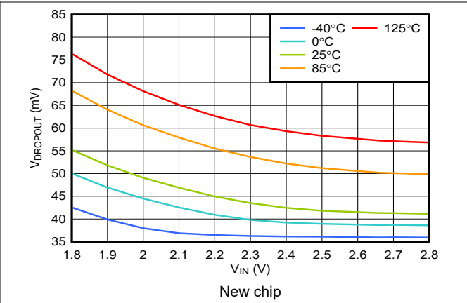
Figure 5-32. TPS793 Dropout Voltage vs Input Voltage
