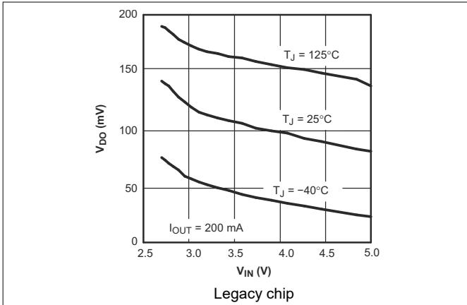
Figure 5-31. TPS793 Dropout Voltage vs Input Voltage
