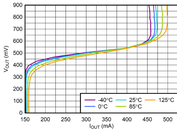
Figure 6-9. Foldback Current Limit vs I_{\text{OUT}}
