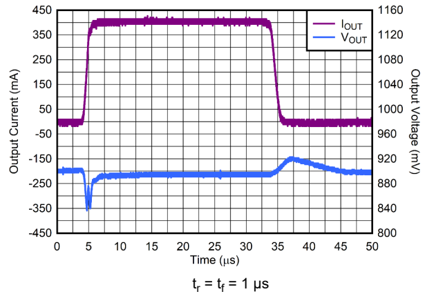
Figure 6-20. Load Transient From 100 \mu\text{A} to 400 mA
