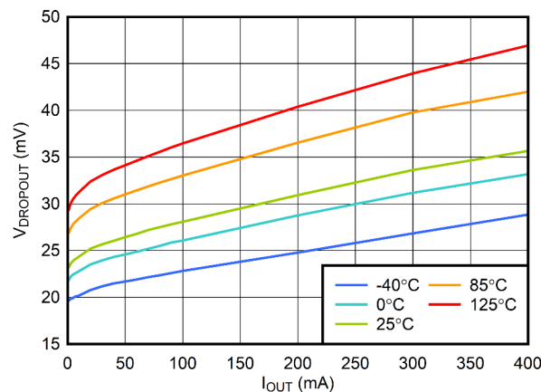
Figure 8-5. V_{\text{IN}} Dropout Voltage vs I_{\text{OUT}}
