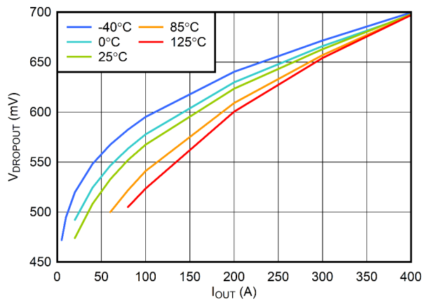
Figure 6-5. V_{\text{BIAS}} Dropout Voltage vs I_{\text{OUT}}
