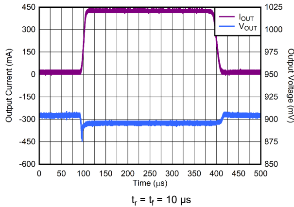
Figure 6-19. Load Transient From 100 \mu\text{A} to 400 mA
