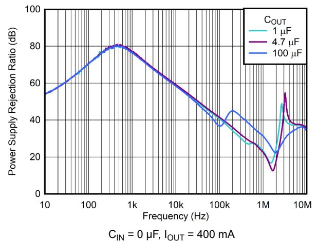
Figure 6-22. V_{IN} PSRR vs Frequency and C_{OUT}
