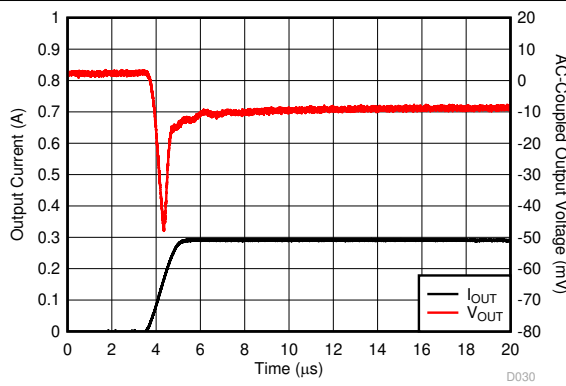
Figure 5-51. Load Transient
