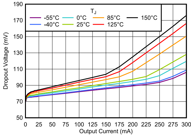
Figure 5-31. Dropout Voltage vs I_{OUT}
