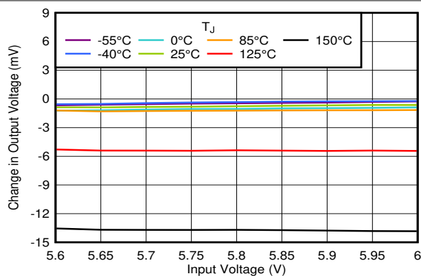
Figure 5-2. Line Regulation vs V_{IN}
