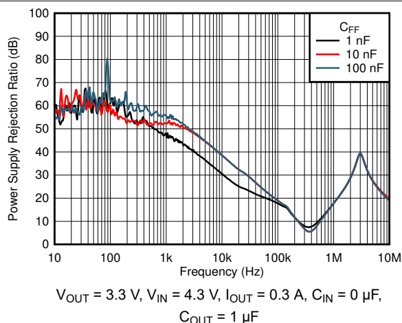
Figure 7-22. PSRR vs Frequency and C_{FF}
