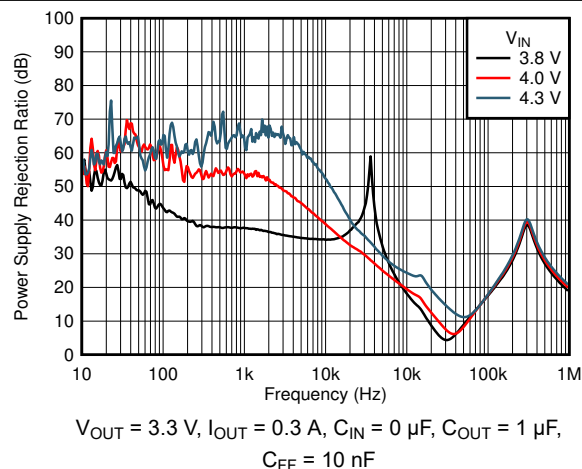
Figure 7-20. PSRR vs Frequency and V_{IN}
