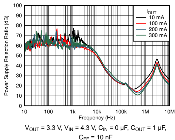
Figure 7-19. PSRR vs Frequency and I_{OUT}
