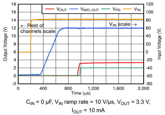
Figure 6-12. Fast Start-Up
