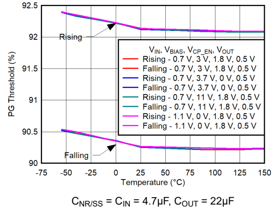
Figure 5-216. PG Threshold Voltage vs Temperature for V_{IN} = 0.7V and 1.1V
