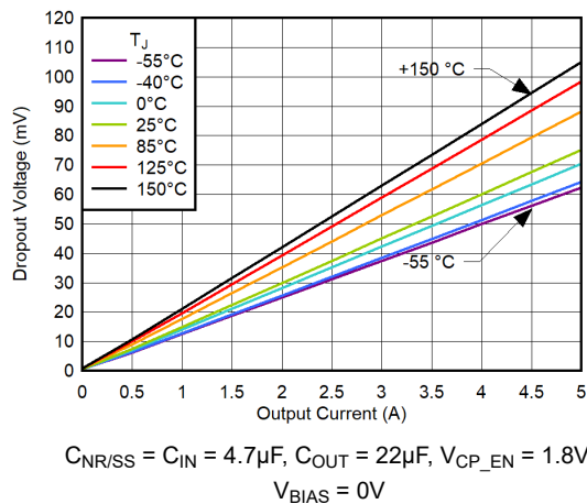
Figure 5-75. Dropout Voltage vs I_{OUT} for CP Enabled, V_{IN} = 6V , No Bias
