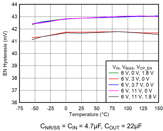
Figure 5-211. EN Hysteresis vs Temperature for V_{IN} = 6V , V_{OUT} = 0.5V
