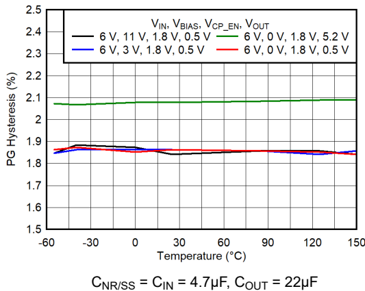
Figure 5-219. PG Hysteresis vs Temperature for V_{IN} = 6V
