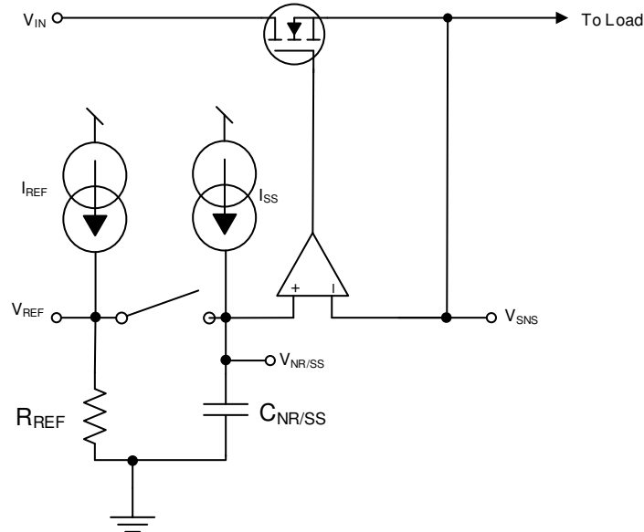
Figure 6-1. Simplified Regulation Circuit
