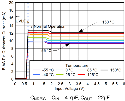
Figure 5-159. BIAS Pin Quiescent Current vs V_{IN} for V_{OUT} = 0.5V , V_{BIAS} = 11V , CP Enabled, I_{OUT} = 0A
