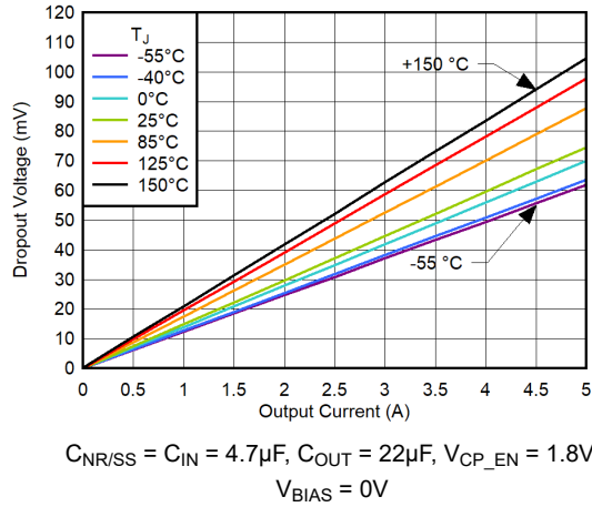
Figure 5-73. Dropout Voltage vs I_{OUT} for CP Enabled, V_{IN} = 1.1V , No Bias
