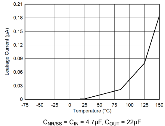
Figure 5-220. PG Leakage Current vs Temperature
