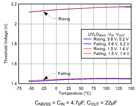
Figure 5-132. UVLO BIAS Threshold vs Temperature for CP Disabled
