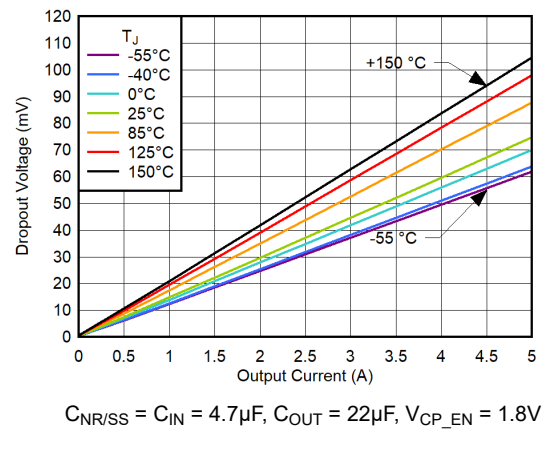
Figure 5-76. Dropout Voltage vs I_{OUT} for CP Enabled, V_{IN} = 5.3V , V_{BIAS} = 3V
