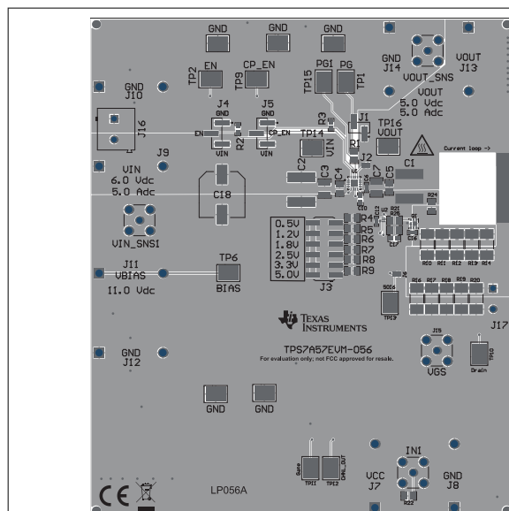
Figure 7-23. Top Assembly Layer and Silkscreen
