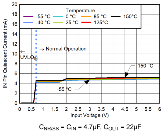
Figure 5-161. IN Pin Quiescent Current vs V_{IN} for V_{OUT} = 0.5V , V_{BIAS} = 11V , CP Enabled, I_{OUT} = 0A
