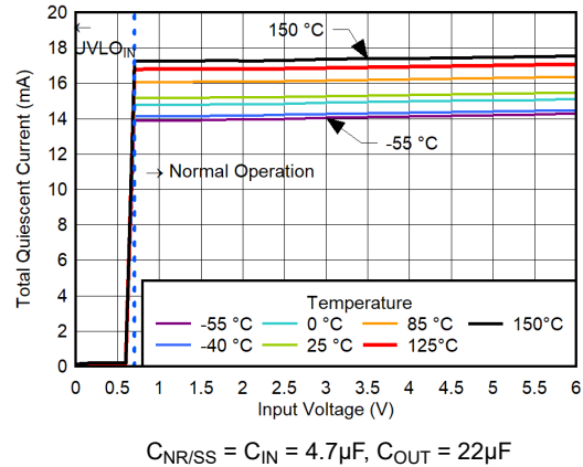
Figure 5-160. Total Quiescent Current vs V_{IN} for V_{OUT} = 0.5V , V_{BIAS} = 11V , CP Enabled, I_{OUT} = 0A
