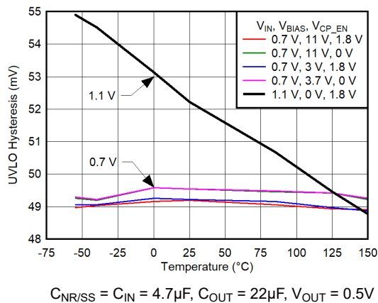
Figure 5-131. UVLO IN Hysteresis vs Temperature
