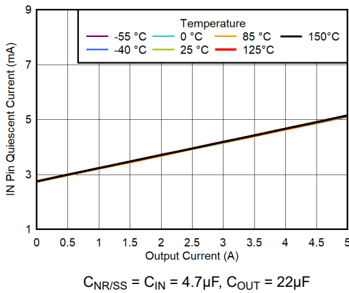
Figure 5-185. IN Pin Quiescent Current vs I_{OUT} for V_{OUT} = 0.5V , V_{IN} = 0.7V , V_{BIAS} = 3.7V , CP Disabled
