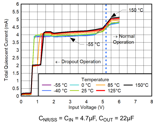
Figure 5-140. Total Quiescent Current vs V_{IN} for V_{OUT} = 5.2V , V_{BIAS} = 8.4V , CP Disabled
