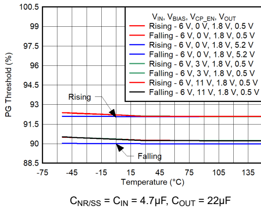
Figure 5-217. PG Threshold Voltage vs Temperature for V_{IN} = 6V
