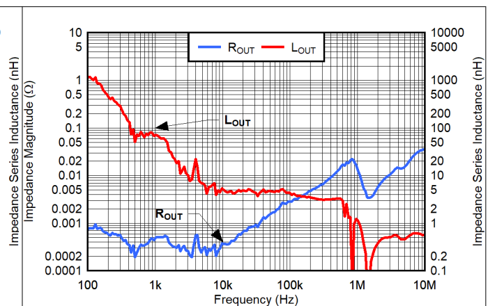
Figure 7-15. V_{IN} = 5.5V , V_{OUT} = 5V , V_{BIAS} = 8V , CP\_EN = 0 , I_{OUT} = 500mA
