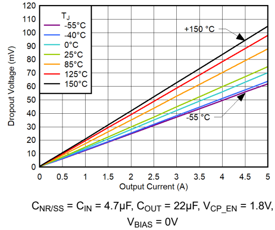
Figure 5-74. Dropout Voltage vs I_{OUT} for CP Enabled, V_{IN} = 5.3V , No Bias
