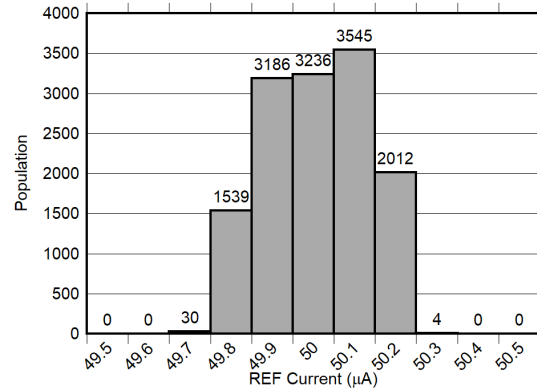
Figure 5-90. I_{REF} Distribution
