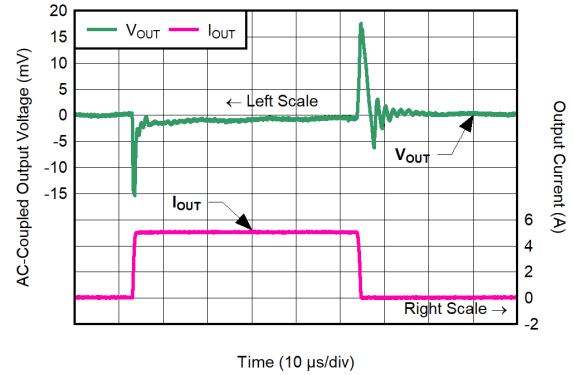
Time (10 \mu s/div ) C_{NR/SS} = C_{IN} = 4.7\mu F , C_{OUT} = 22\mu F , V_{CP\_EN} = 0V , V_{BIAS} = 8.4V , V_{IN} = 5.5V
