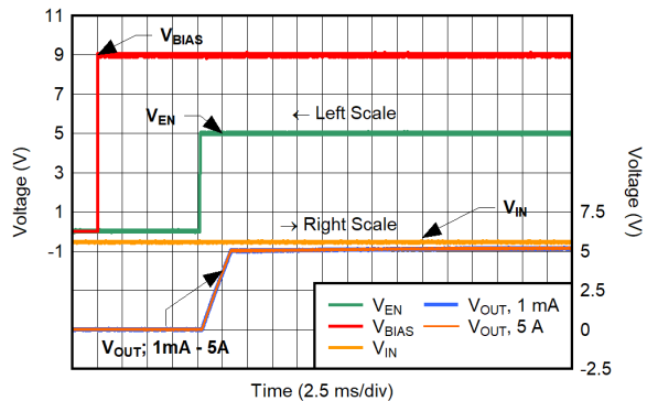
Figure 5-58. Start-Up for CP_EN-BIAS-IN Rail Sequence for CP Enabled
