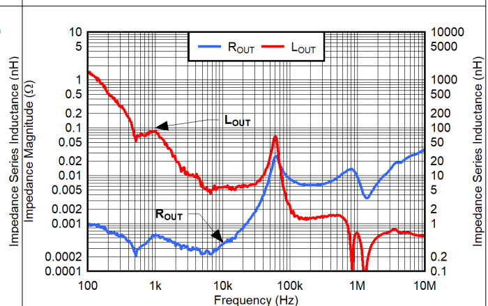
Figure 7-17. V_{IN} = 0.9V , V_{BIAS} = 3V , V_{OUT} = 0.5V , CP\_EN = 0 , I_{OUT} = 4.6A
