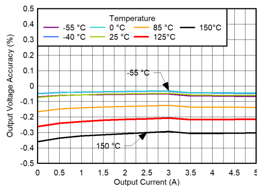
Figure 5-106. Output Voltage Accuracy vs I_{OUT} for V_{IN} = 1.1V , CP Enabled
