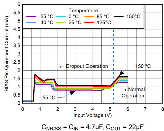
Figure 5-138. BIAS Pin Quiescent Current vs V_{IN} for V_{OUT} = 5.2V , V_{BIAS} = 8.4V , CP Disabled
