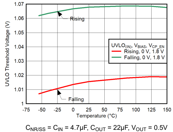
Figure 5-130. UVLO IN Threshold vs Temperature Without BIAS Rail
