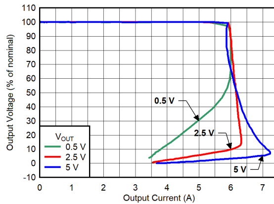
Figure 7-10. Current Limit Foldback Behavior
