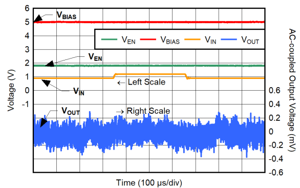
Time (100 \mu s/div ) C_{NR/SS} = C_{IN} = 4.7\mu F , C_{OUT} = 22\mu F , V_{CP\_EN} = 0V , V_{BIAS} = 5V , V_{OUT} = 0.5V , I_{OUT} = 100mA , SR = 1V/\mu s
