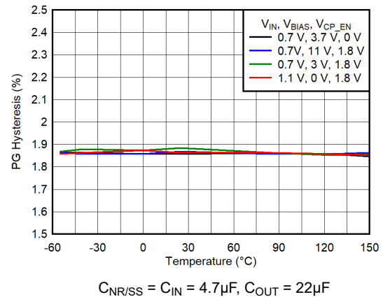
Figure 5-218. PG Hysteresis vs Temperature for V_{IN} = 0.7V and 1.1V
