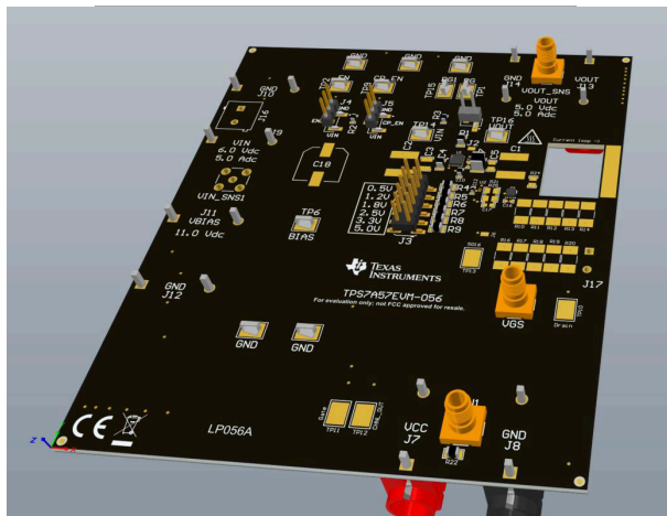
Figure 7-31. TPS7A57EVM-056 3D View
