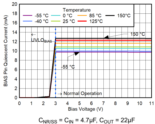
Figure 5-162. BIAS Pin Quiescent Current vs V_{BIAS} for V_{OUT} = 0.5V , V_{IN} = 0.7V , CP Enabled, I_{OUT} = 0A
