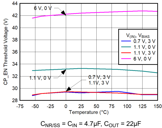
Figure 5-215. CP_EN Hysteresis vs Temperature
