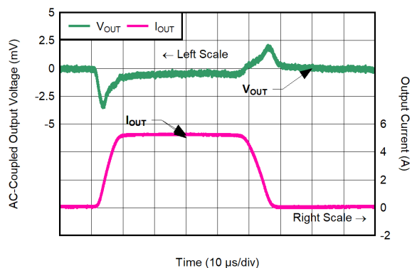
Figure 5-33. Load Transient for V_{OUT} = 0.5V , I_{OUT} = 100mA to 5 A, CP Enabled
