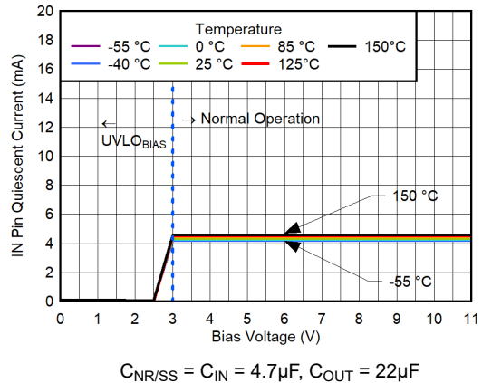
Figure 5-164. IN Pin Quiescent Current vs V_{BIAS} for V_{OUT} = 0.5V , V_{IN} = 0.7V , CP Enabled, I_{OUT} = 0A
