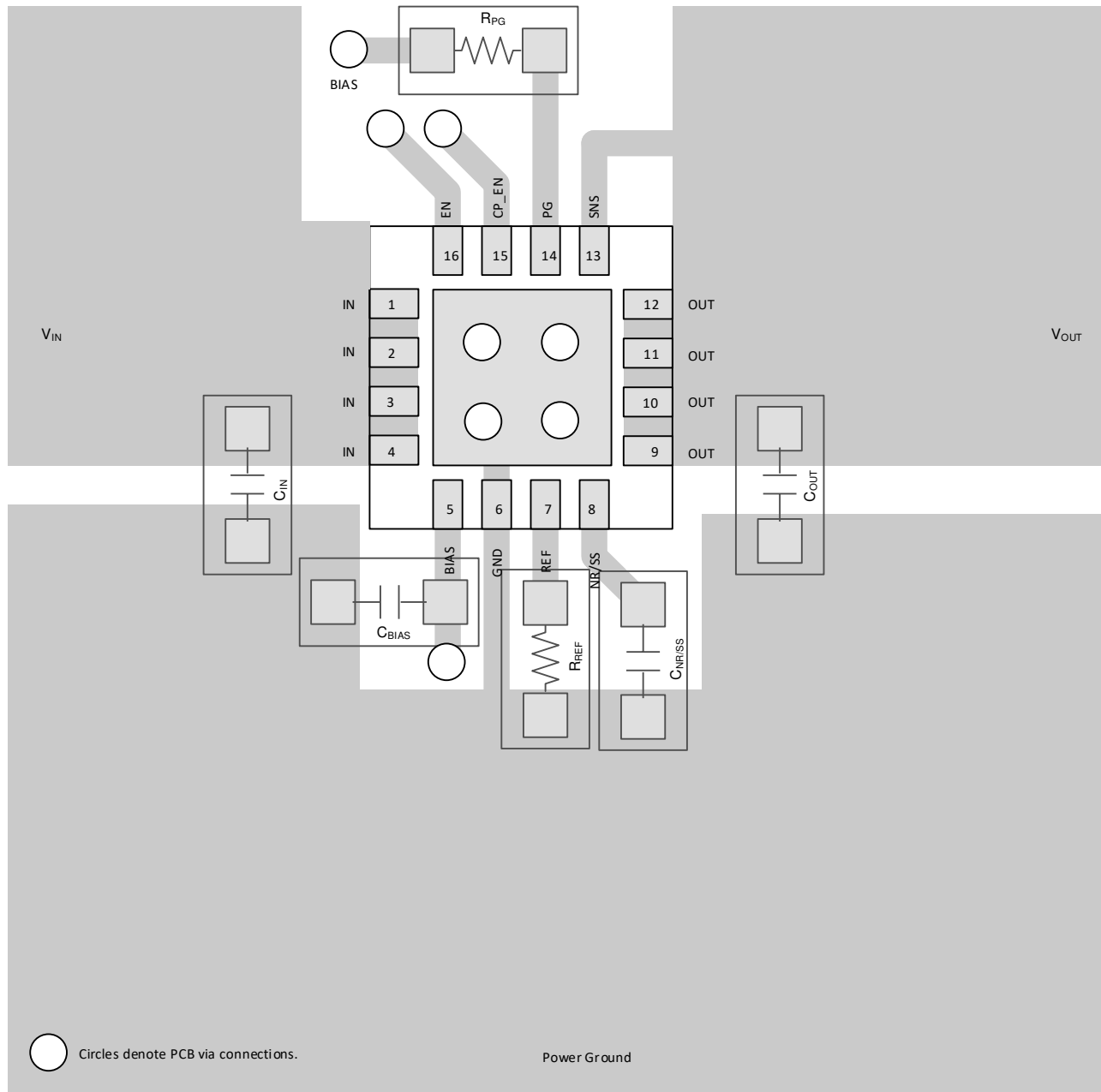
Figure 7-38. Recommended Layout
