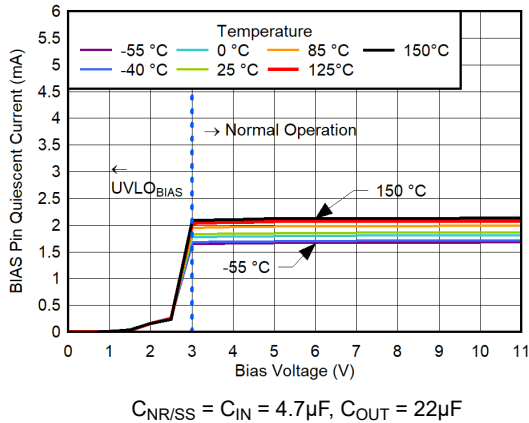
Figure 5-177. BIAS Pin Quiescent Current vs V_{BIAS} for V_{OUT} = 0.5V , V_{IN} = 0.7V , CP Disabled, I_{OUT} = 0A
