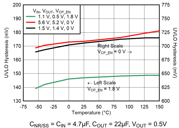
Figure 5-134. UVLO IN Hysteresis vs Temperature
