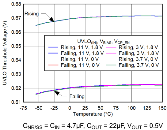
Figure 5-129. UVLO IN Threshold vs Temperature With BIAS Rail
