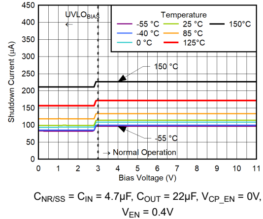
Figure 5-206. IN Pin Shutdown Current vs V_{BIAS} for V_{IN} = 6V , V_{OUT(nom)} = 0.5V , CP Disabled
