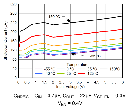
Figure 5-192. Total Shutdown Current vs V_{IN} for V_{OUT} = 0.5V , V_{BIAS} = 11V , CP Disabled
