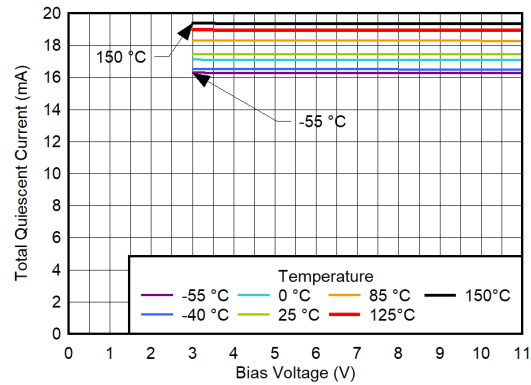
Figure 5-166. Total Quiescent Current vs V_{BIAS} for V_{OUT} = 0.5V , V_{IN} = 0.7V , CP Enabled, I_{OUT} = 5A
