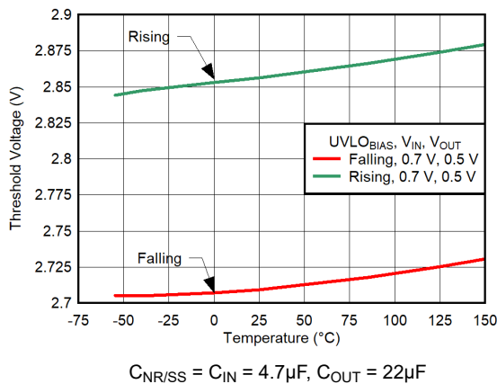
Figure 5-133. UVLO BIAS Threshold vs Temperature for CP Enabled
