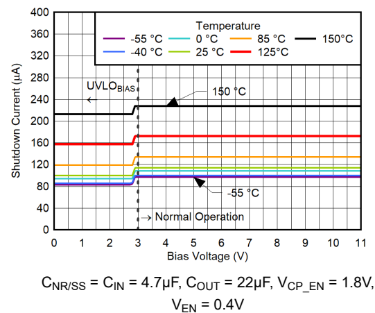
Figure 5-200. IN Pin Shutdown Current vs V_{BIAS} for V_{IN} = 6V , V_{OUT(nom)} = 0.5V , CP Enabled
