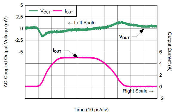
Time (10 \mu s/div ) C_{NR/SS} = C_{IN} = 4.7\mu F , C_{OUT} = 22\mu F , V_{CP\_EN} = 0V , V_{BIAS} = 8.4V , V_{IN} = 5.5V
