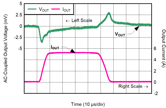
Time (10 \mu s/div ) C_{NR/SS} = C_{IN} = 4.7\mu F , C_{OUT} = 22\mu F , V_{CP\_EN} = 0V , V_{BIAS} = 6.5V , V_{IN} = 3.6V
