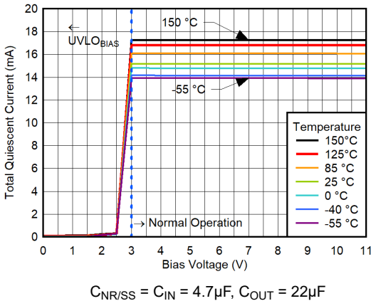
Figure 5-163. Total Quiescent Current vs V_{BIAS} for V_{OUT} = 0.5V , V_{IN} = 0.7V , CP Enabled, I_{OUT} = 0A
