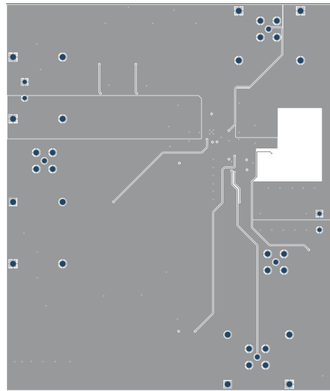
Figure 7-26. Layer 3 Routing
