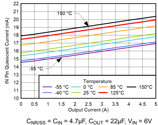
Figure 5-152. IN Pin Quiescent Current vs I_{OUT} for V_{OUT} = 5.2V , CP Enabled
