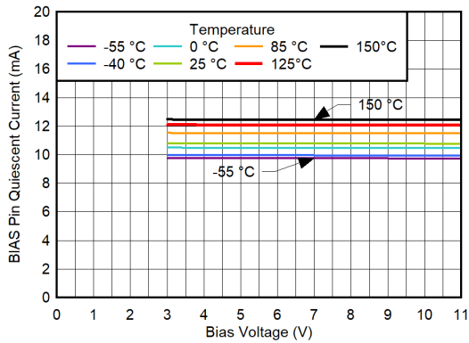
Figure 5-165. BIAS Pin Quiescent Current vs V_{BIAS} for V_{OUT} = 0.5V , V_{IN} = 0.7V , CP Enabled, I_{OUT} = 5A
