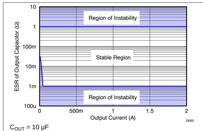
Figure 1. Stability Curve
