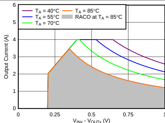
Figure 60. Recommended Area for Continuous Operation for V_{OUTX} = 1.2\text{ V}
