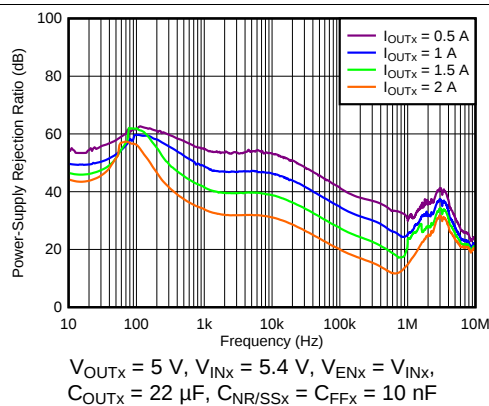
Figure 3. Power-Supply Rejection Ratio vs Frequency and Output Current
