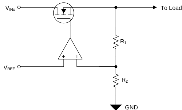
Figure 44. Simplified Regulation Circuit
