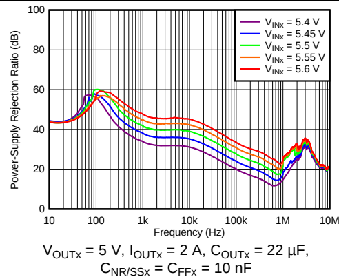
Figure 2. Power-Supply Rejection Ratio vs Frequency and Input Voltage
