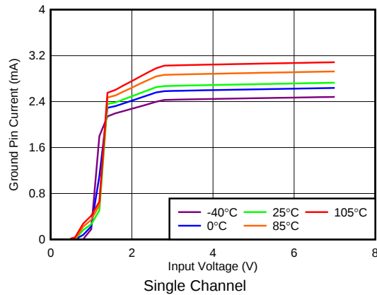
Figure 31. Ground Current vs Input Voltage
