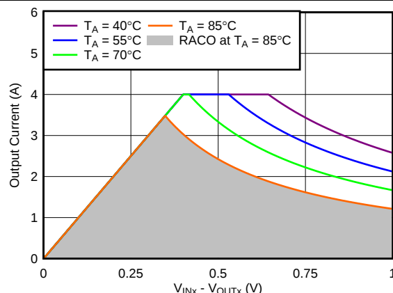
Figure 64. Recommended Area for Continuous Operation for V_{OUTX} = 5.0\text{ V}
