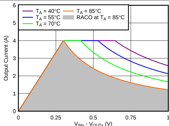
Figure 63. Recommended Area for Continuous Operation for V_{OUTX} = 3.3\text{ V}
