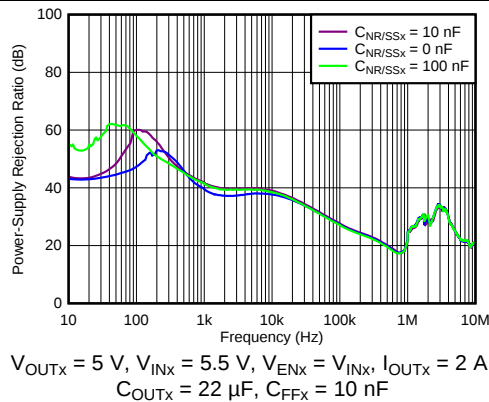
Figure 1. Power-Supply Rejection Ratio vs Frequency and C_{NR/SSx}
