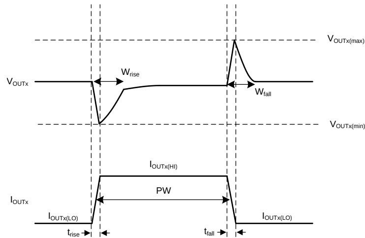
Figure 54. Simplified Load Transient Waveform
