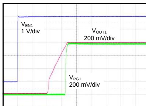
Figure 40. Start-Up (SS_CTRLX = GND, C_{\text{NR/SSx}} = 0\text{ nF} )
