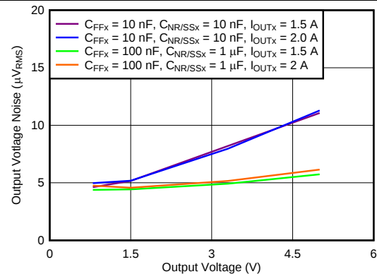
Figure 8. Output Noise vs Output Voltage
