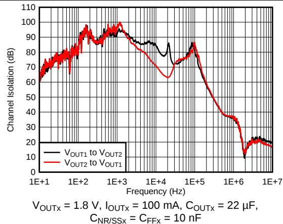
Figure 7. Channel-to-Channel Output Voltage Isolation vs Frequency
