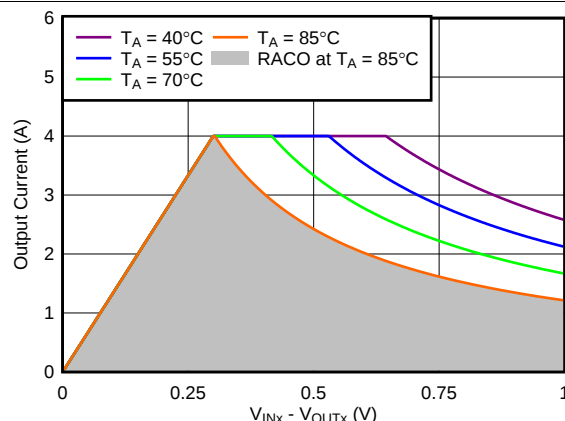
Figure 62. Recommended Area for Continuous Operation for V_{OUTX} = 2.5\text{ V}
