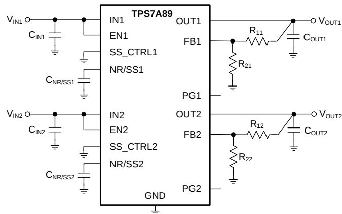
Figure 48. Adjustable Operation
