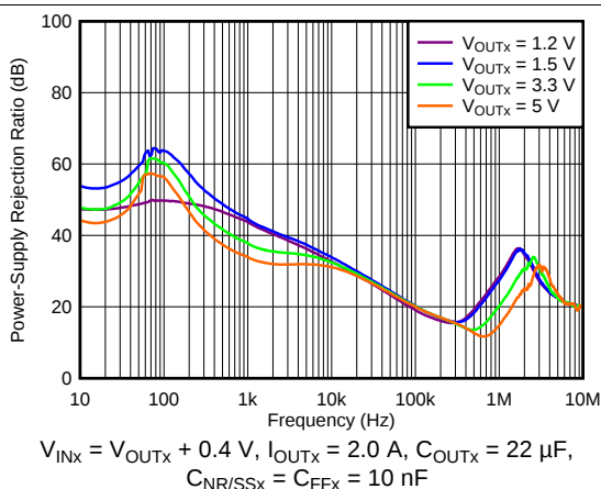
Figure 5. Power-Supply Rejection Ratio vs Frequency and Output Voltage
