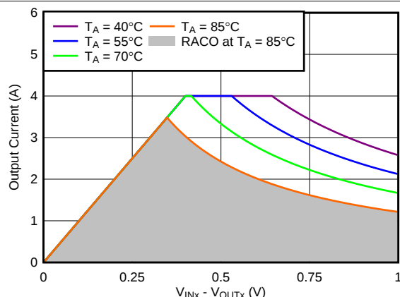
Figure 61. Recommended Area for Continuous Operation for V_{OUTX} = 1.8\text{ V}
