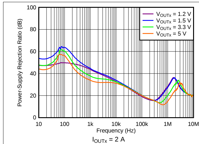
Figure 66. Power-Supply Rejection Ratio vs Frequency
