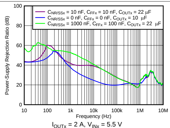
Figure 4. Power-Supply Rejection Ratio vs Frequency and Output Capacitance
