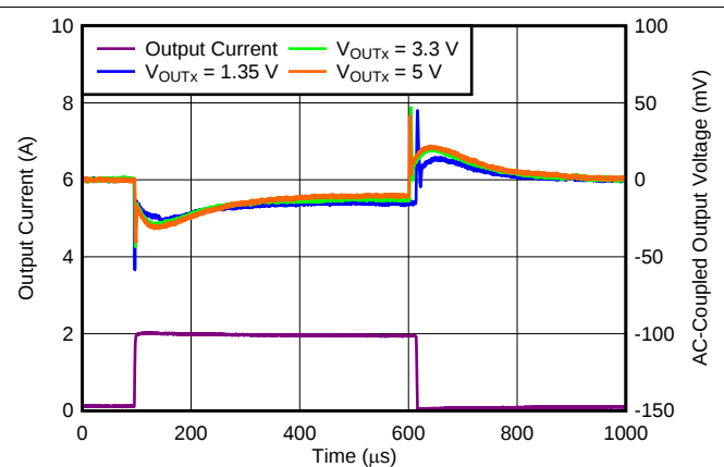
Figure 67. Load Transient Response vs Time and V_{OUTx}
