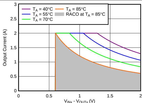
Figure 59. Recommended Area for Continuous Operation for V_{OUTX} = 0.8\text{ V}
