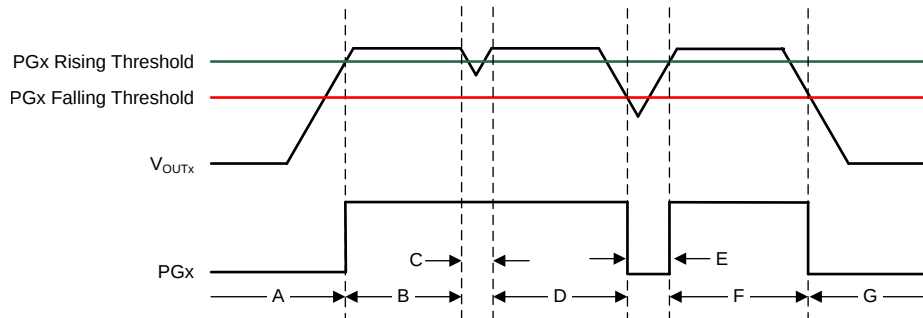
Figure 50. Typical PGx Operation
