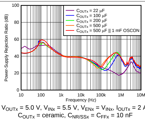
Figure 4. Power-Supply Rejection Ratio vs Frequency and Output Capacitance
