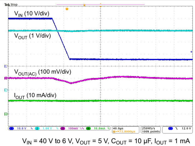
Figure 5-16. Line Transient
