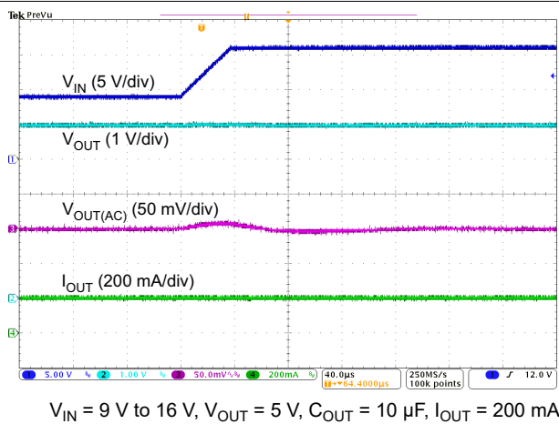
Figure 5-17. Line Transient
