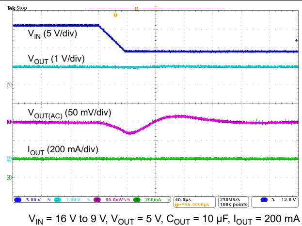
Figure 5-18. Line Transient
