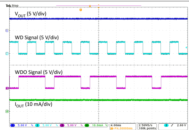
Figure 7-3. TPS7B6350-Q1 Watchdog Fault (High-Frequency Watchdog Service Signal)
