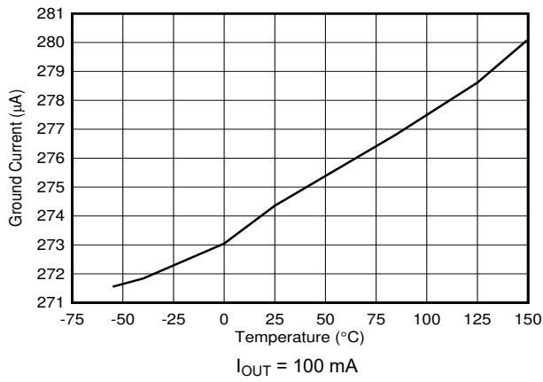
Figure 6-25. Ground Current
