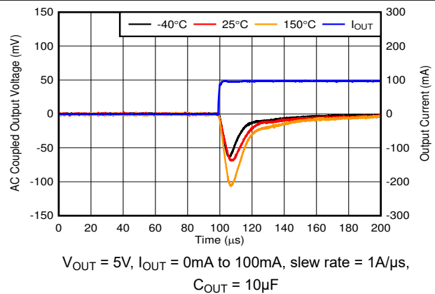
Figure 5-16. Load Transient, No Load to 100mA Rising Edge
