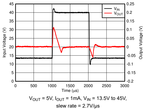
Figure 5-13. Line Transients
