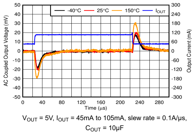
Figure 5-17. Load Transient, 45mA to 105mA
