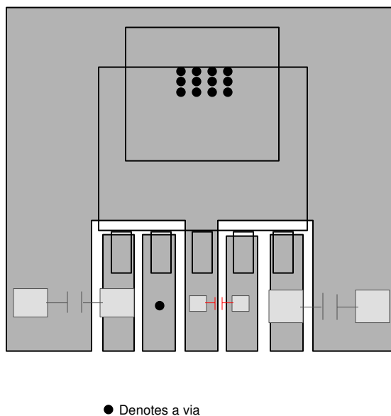
Figure 7-12. KVV Package Fixed Output
