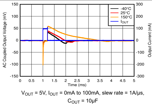
Figure 5-15. Load Transient, No Load to 100mA
