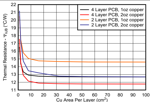
Figure 7-3. \psi_{JB} vs Copper Area (DDA Package)
