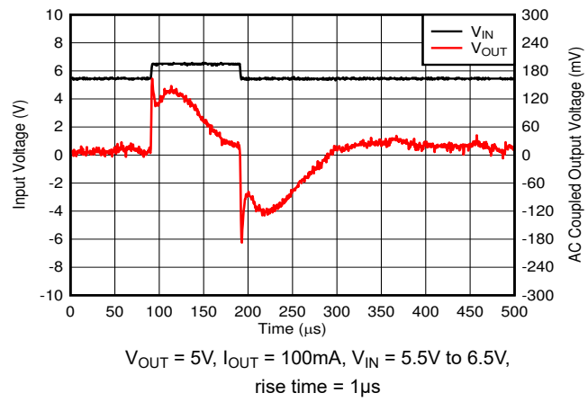
Figure 5-14. Line Transients
