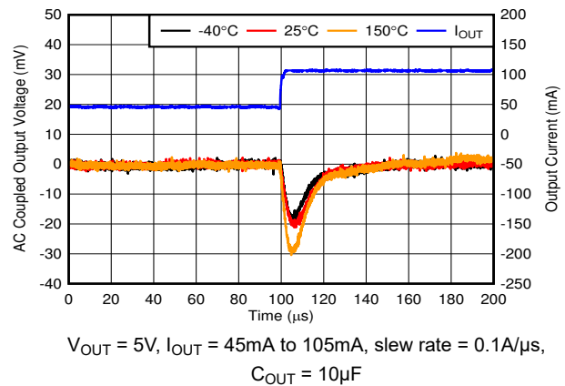
Figure 5-18. Load Transient, 45mA to 105mA Rising Edge
