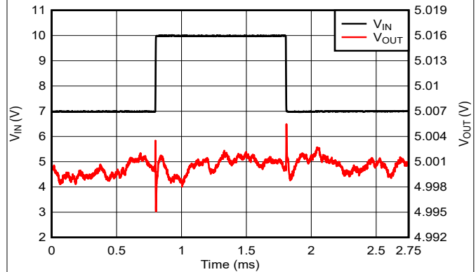
Figure 5-20. V_{IN} Line Transient (7V to 10V)
