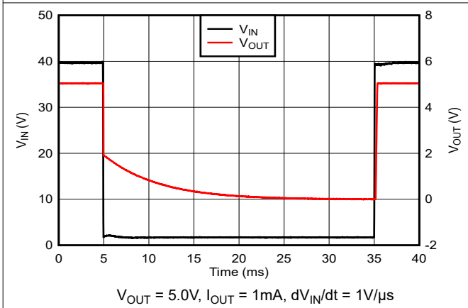
Figure 7-12. Brownout Transient (40V to 1.7V)
