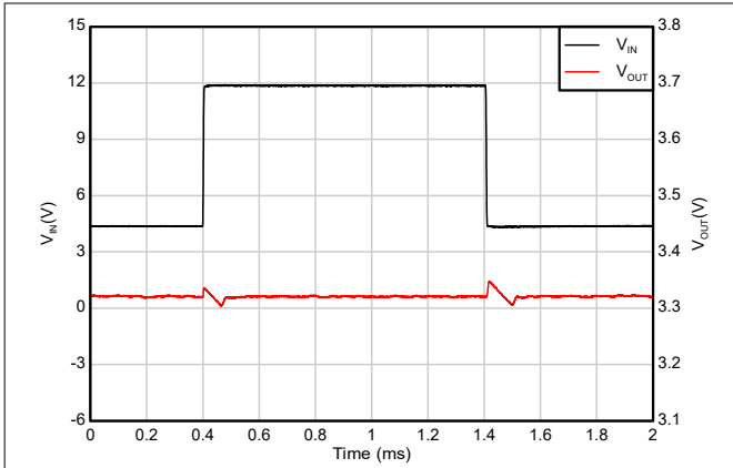
Figure 5-43. Line Transient (4.3V to 12V)
