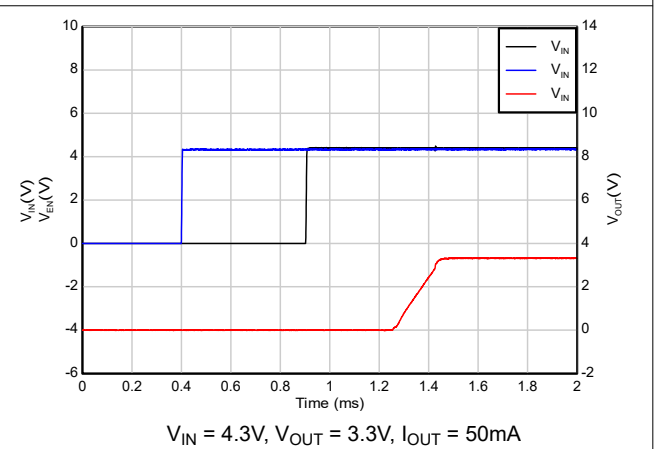
Figure 5-40. Start-up with sequencing ( V_{IN} after EN)
