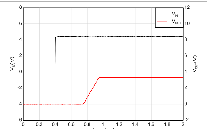
Figure 7-6. Start-up with EN & V_{IN} tied together
