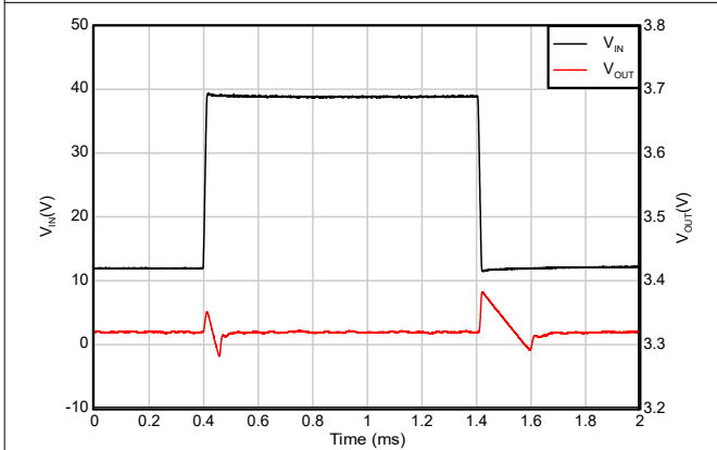
Figure 5-45. Line Transient (12V to 40V)
