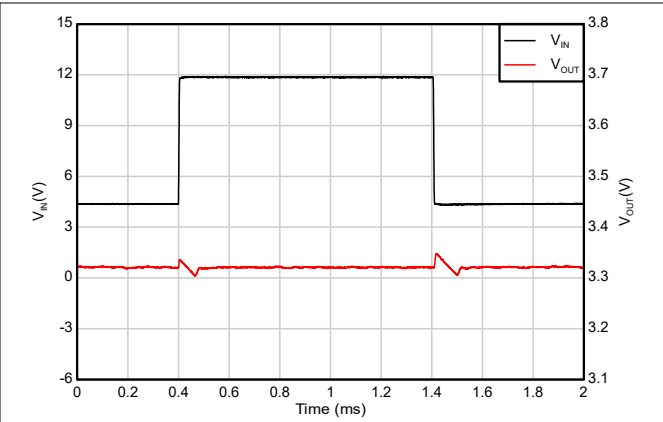
Figure 5-44. Line Transient (4.3V to 12V)
