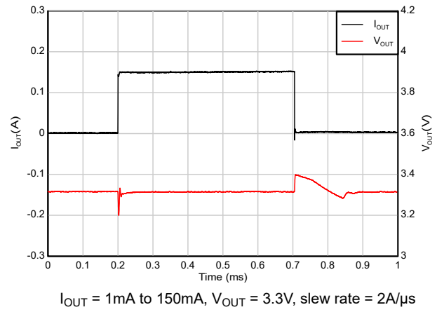
Figure 7-7. Load Transient
