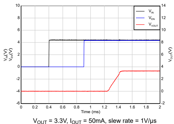
Figure 7-8. Start-up With Sequencing (EN after IN)
