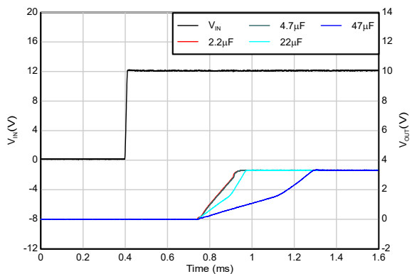
Figure 5-50. Start-up With IN and EN Tied Together, C_{OUT}
