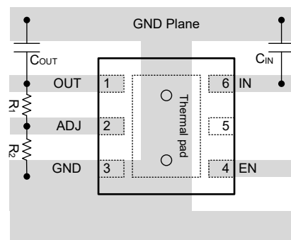
Figure 7-12. Example Layout for TPS7E72 DRV Package
