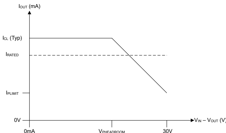
Figure 6-4. Power Limiting
