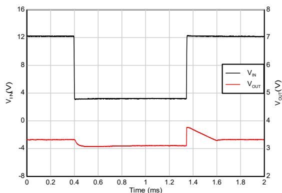
Figure 5-39. Dropout Recovery
