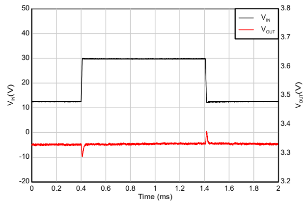
Figure 5-32. Line Transient
