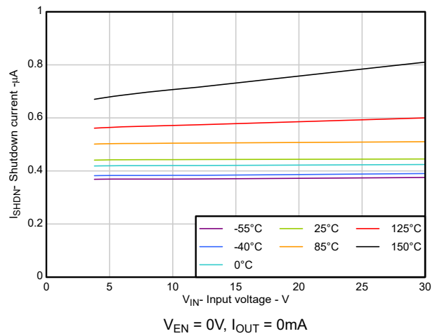
Figure 5-14. Shutdown Current vs Input Voltage
