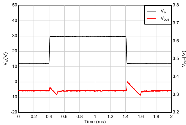
Figure 5-31. Line Transient
