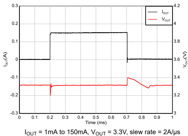
Figure 7-7. Load Transient
