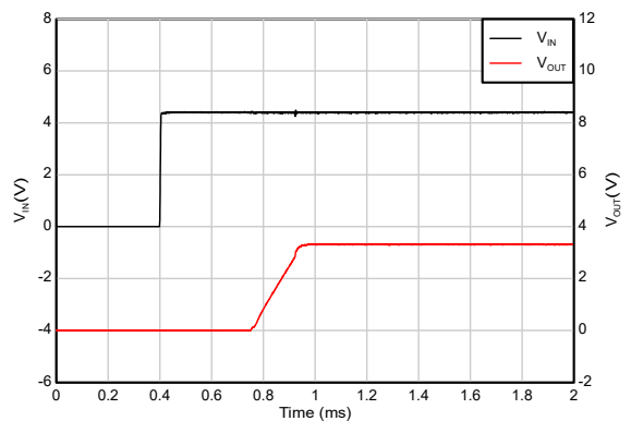
Figure 5-49. Start-up With IN and EN Tied Together
