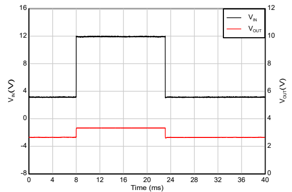
Figure 5-32. Line Transient
