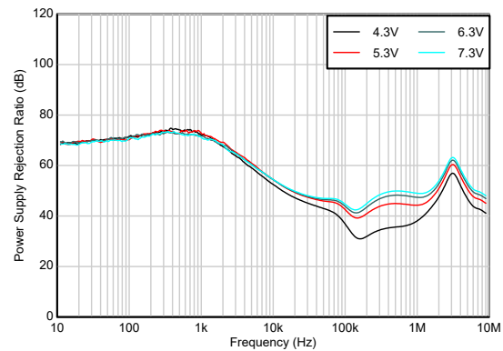
Figure 5-20. Ripple Rejection vs Frequency, Input Voltage
