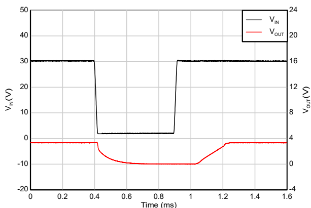
Figure 5-40. Dropout Recovery
