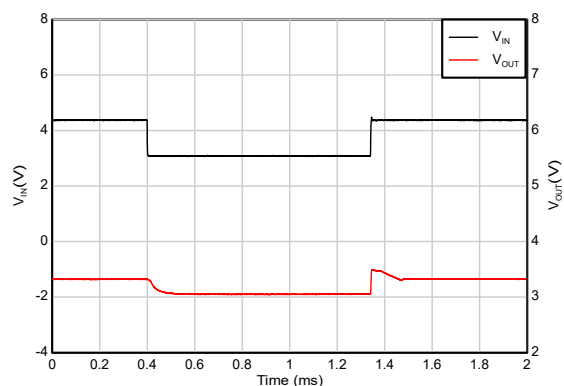
Figure 5-37. Dropout Recovery
