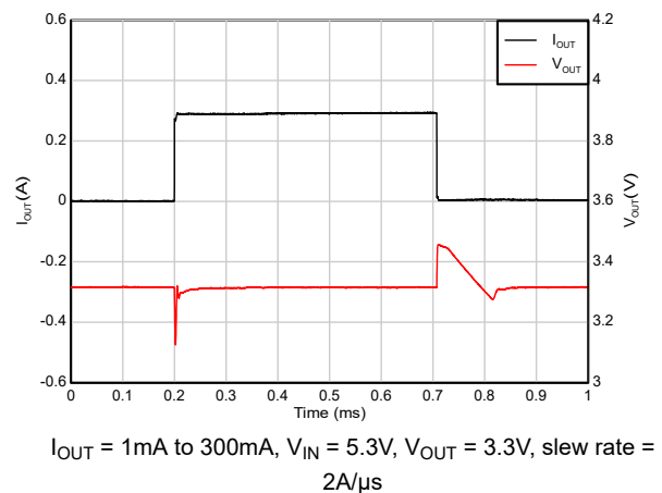
Figure 5-36. Load Transient
