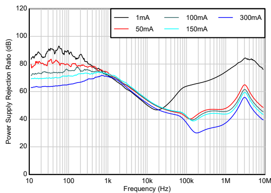
Figure 5-19. Ripple Rejection vs Frequency, C_{OUT}
