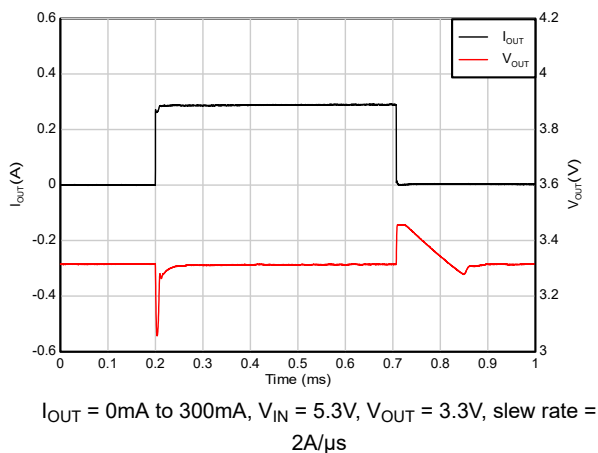
Figure 5-35. Load Transient
