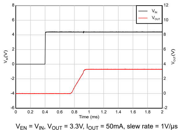
Figure 7-10. Start-up With IN and EN Tied Together
