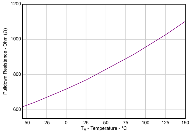
Figure 5-17. Pull-down Resistance on Output ( R_{\text{Discharge}} ) vs Temperature
