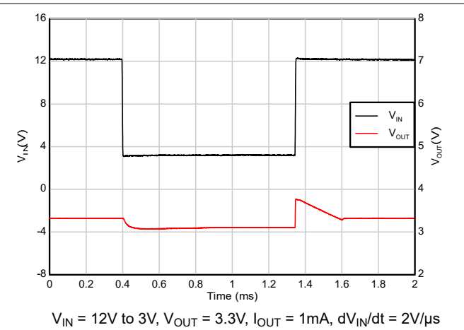
Figure 5-48. Dropout Recovery (12V to 3V)
