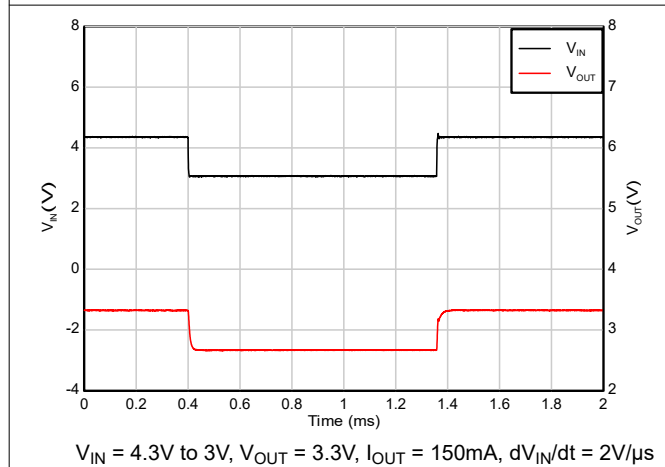
Figure 5-47. Dropout Recovery (4.3V to 3V)
