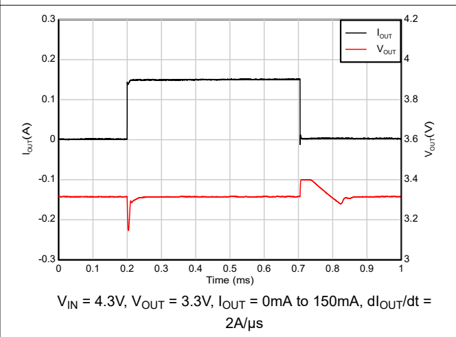
Figure 5-44. Load Transient (0mA to 150mA)
