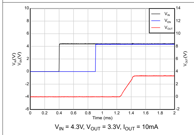
Figure 5-35. Start-up with sequencing (EN after V_{IN} )
