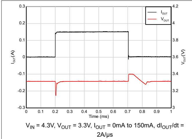
Figure 7-13. Load Transient (0mA to 150mA)
