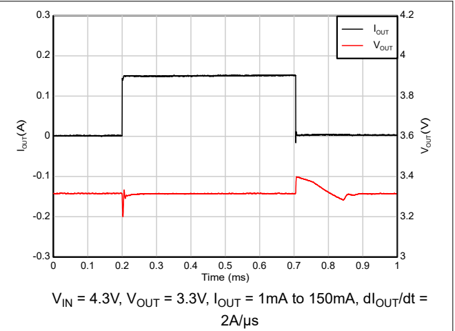
Figure 7-14. Load Transient (1mA to 150mA)
