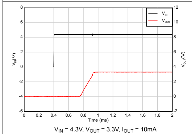
Figure 7-9. Start-up with EN & V_{IN} tied together
