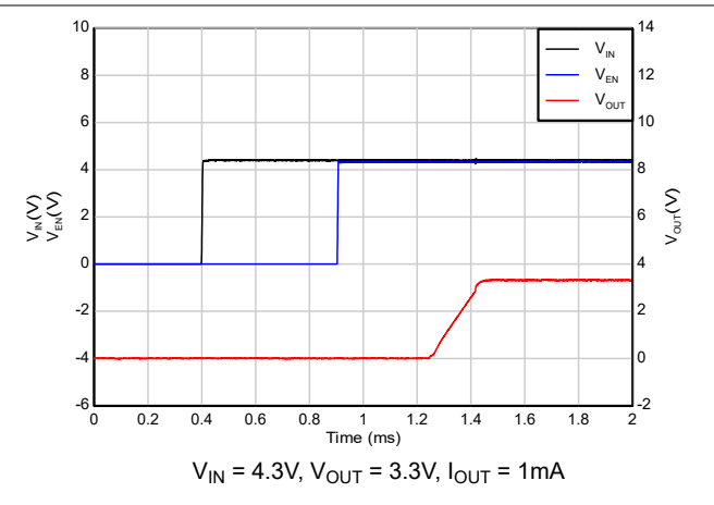
Figure 5-34. Start-up with sequencing (EN after V_{IN} )
