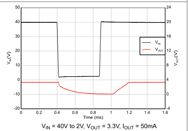
Figure 7-18. Brown-out Recovery (40V to 2V)
