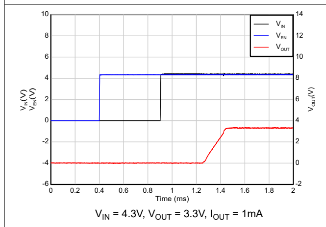
Figure 5-37. Start-up with sequencing ( V_{IN} after EN)
