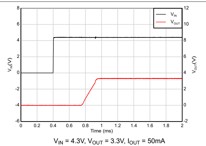
Figure 7-10. Start-up with EN & V_{IN} tied together
