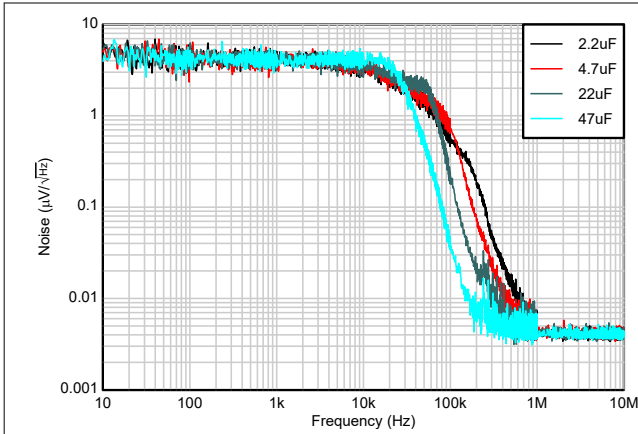
Figure 5-27. Noise vs C_{OUT}
