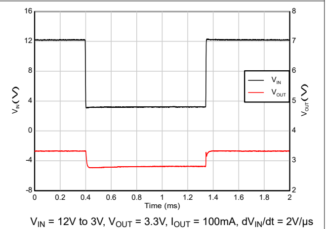
Figure 7-16. Dropout Recovery (12V to 3V)
