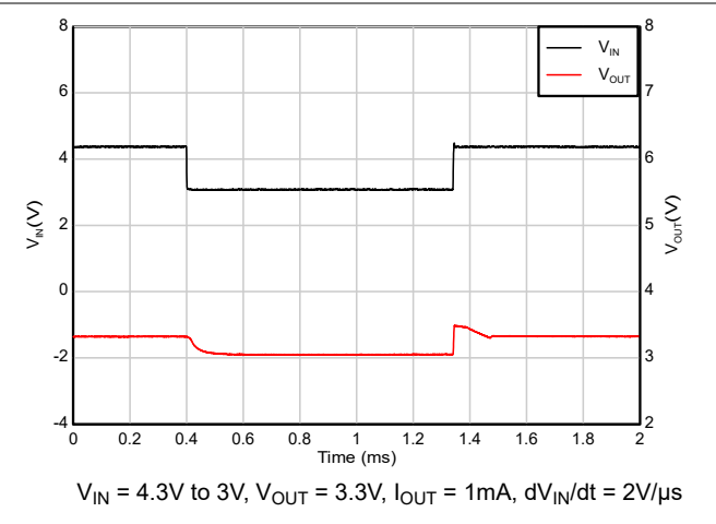
Figure 5-46. Dropout Recovery (4.3V to 3V)
