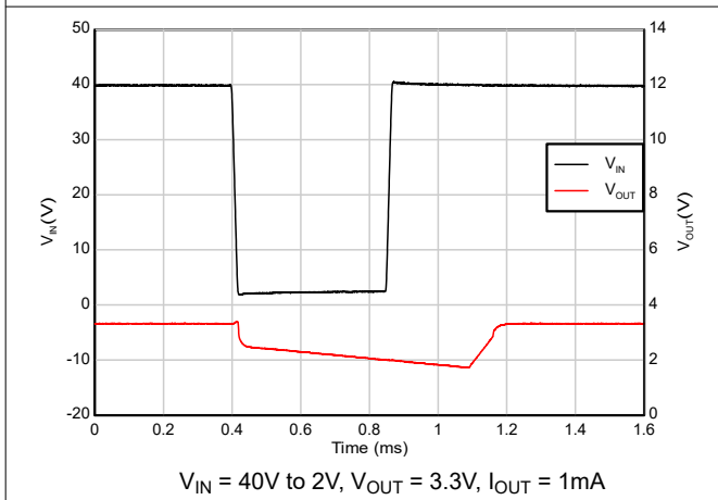
Figure 7-17. Brown-out Recovery (40V to 2V)
