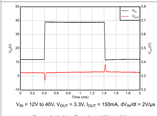
Figure 5-43. Line Transient (12V to 40V)
