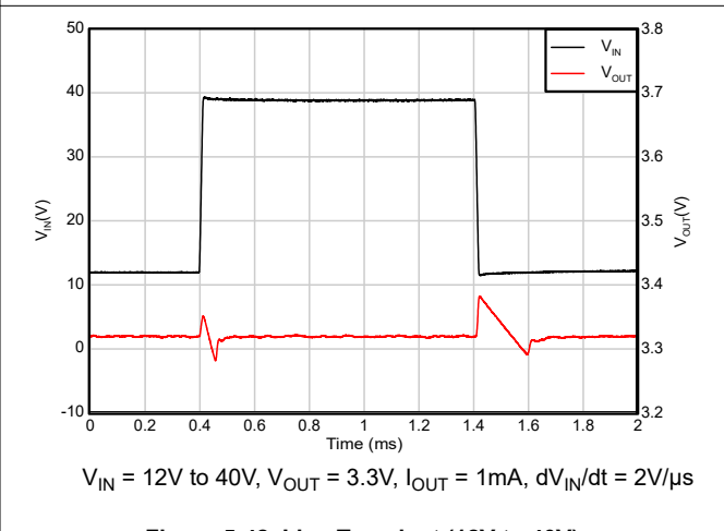
Figure 5-42. Line Transient (12V to 40V)
