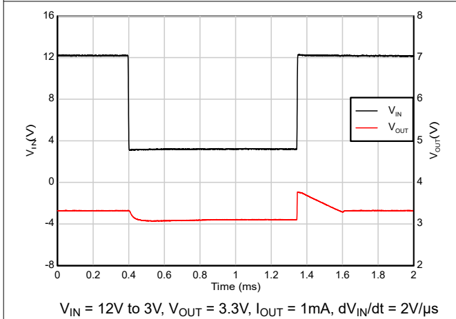
Figure 7-15. Dropout Recovery (12V to 3V)
