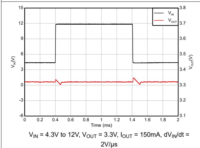
Figure 5-41. Line Transient (4.3V to 12V)
