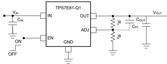
Figure 3-1. Typical Application
