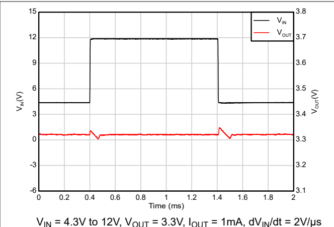
Figure 5-40. Line Transient (4.3V to 12V)
