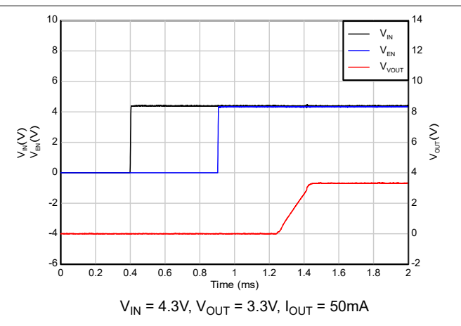
Figure 5-36. Start-up with sequencing (EN after V_{IN} )
