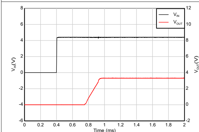
Figure 5-29. Start-up vs C_{OUT}
