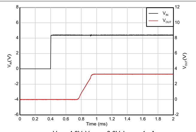
Figure 7-8. Start-up with EN & V_{IN} tied together
