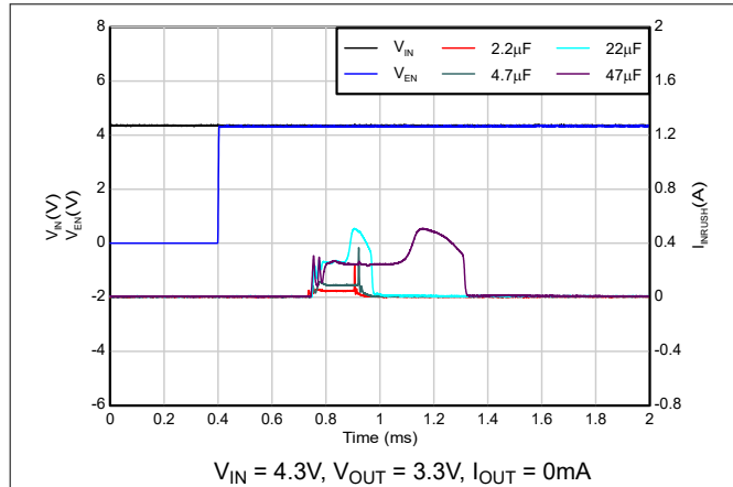
Figure 7-7. Inrush Current vs C_{OUT}
