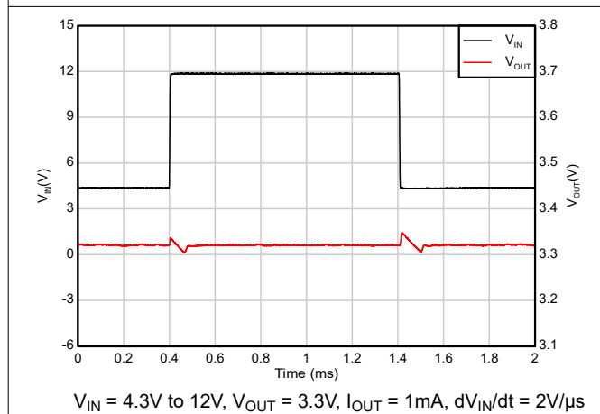
Figure 7-11. Line Transient (4.3V to 12V)
