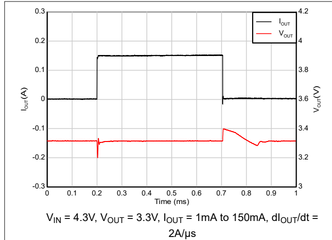
Figure 5-45. Load Transient (1mA to 150mA)
