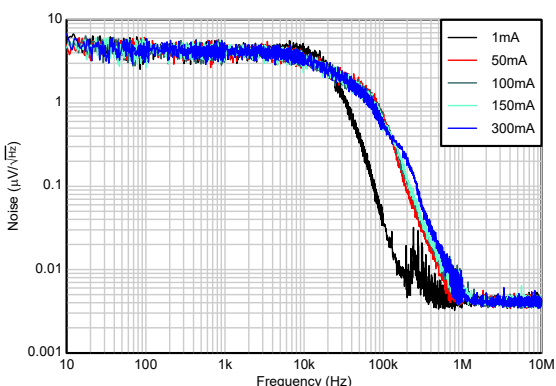
Figure 5-23. Output Noise vs Frequency, C_{OUT}
