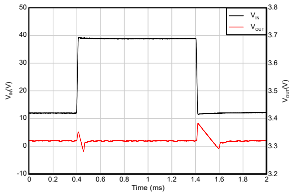
Figure 5-31. Line Transient
