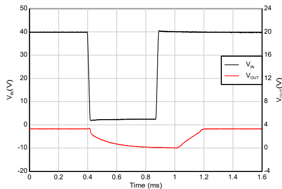
Figure 5-40. Dropout Recovery
