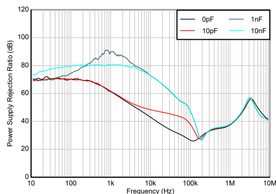
Figure 5-22. Ripple Rejection vs Frequency, C_{FF}
