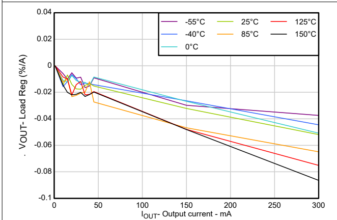
Figure 5-5. Load Regulation
