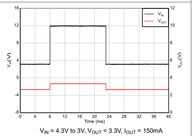
Figure 5-48. Cold-crank Recovery
