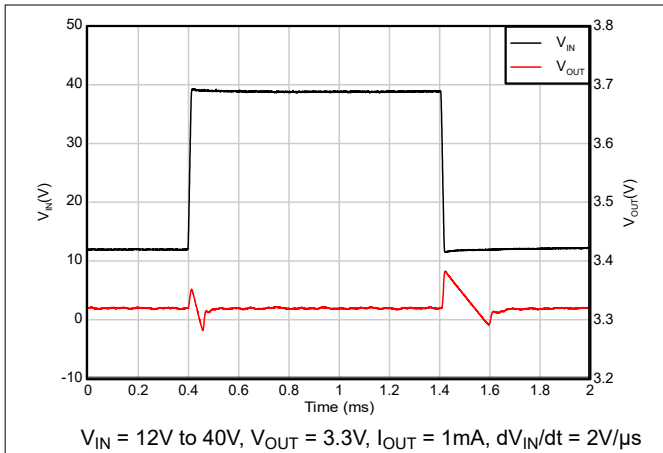
Figure 5-39. Line Transient (12V to 40V)
