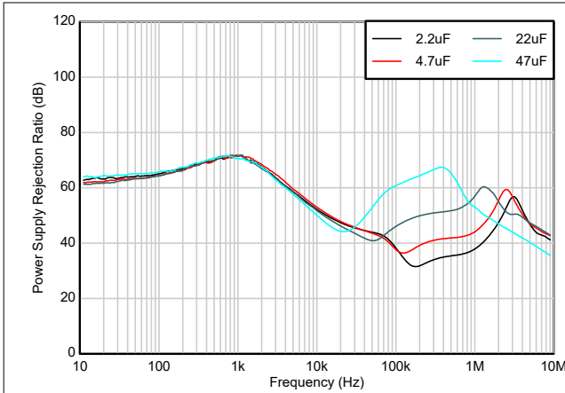
Figure 5-21. PSRR vs C_{OUT}
