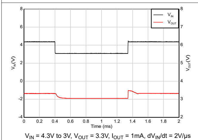
Figure 5-43. Dropout Recovery (4.3V to 3V)
