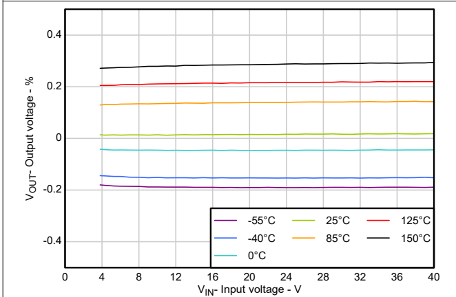
Figure 5-3. V_{OUT} Accuracy vs V_{IN}
