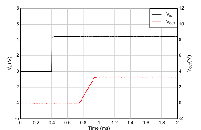
V_{IN} = 4.3\text{V} , V_{OUT} = 3.3\text{V} , I_{OUT} = 50\text{mA}
