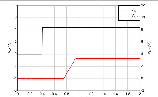
V_{IN} = 4.3\text{V} , V_{OUT} = 3.3\text{V} , I_{OUT} = 1\text{mA} Figure 7-8. Start-up with EN & V_{IN} tied together
