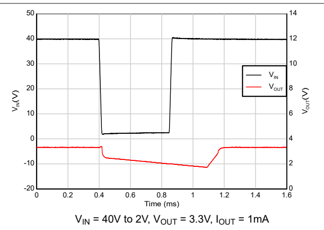
Figure 7-16. Brown-out Recovery (40V to 2V)
