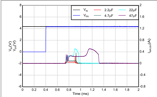
V_{IN} = 4.3\text{V} , V_{OUT} = 3.3\text{V} , I_{OUT} = 0\text{mA} Figure 7-7. Inrush Current vs C_{OUT}
