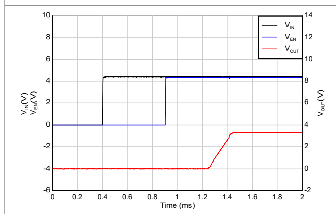
V_{IN} = 4.3\text{V} , V_{OUT} = 3.3\text{V} , I_{OUT} = 1\text{mA}
