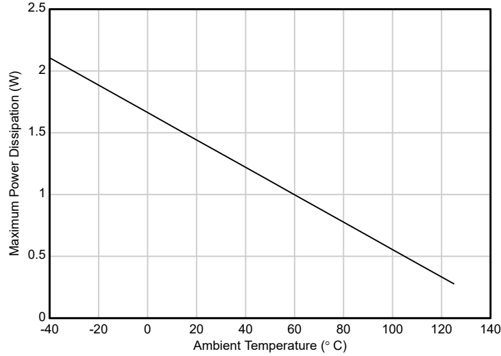
Figure 7-3. TPS7E82-Q1 (DRV) Allowable Power Dissipation
