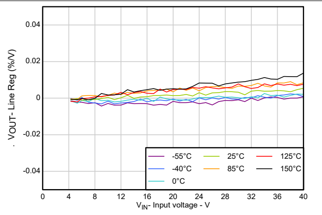
Figure 5-4. Line Regulation
