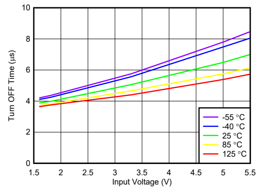
Figure 6-18. Turn OFF Time vs Input Voltage
