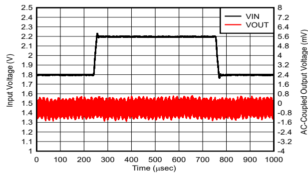
Figure 5-13. IN Line Transient for V_{IN} = 1.8\ V to 2.2\ V
