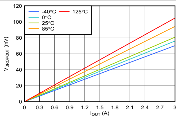
Figure 5-17. Dropout Voltage vs I_{OUT}
