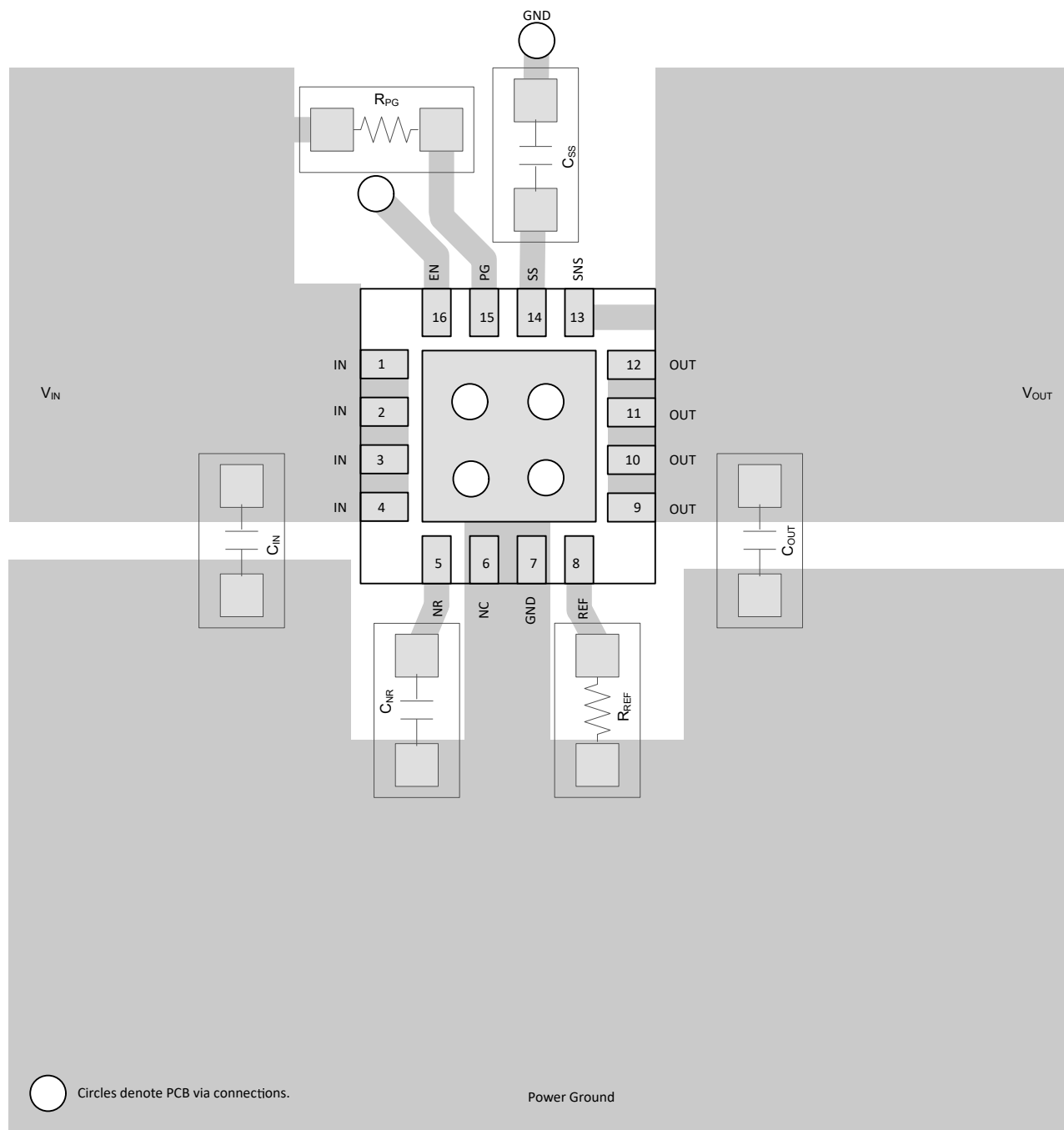
Figure 7-11. Recommended Layout
