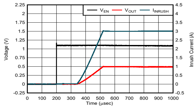
Figure 5-15. Inrush Current for V_{OUT} = 0.5V
