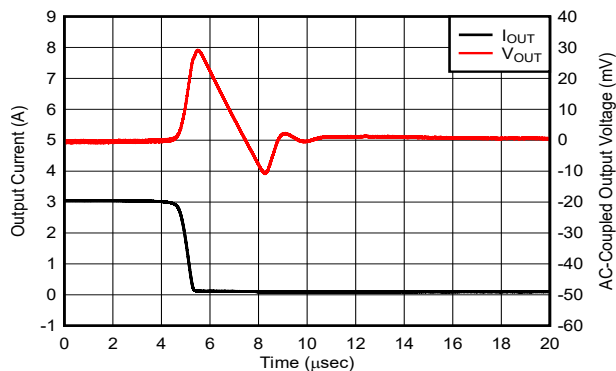
Figure 5-9. Load Transient for I_{OUT} = 3A to 0A
