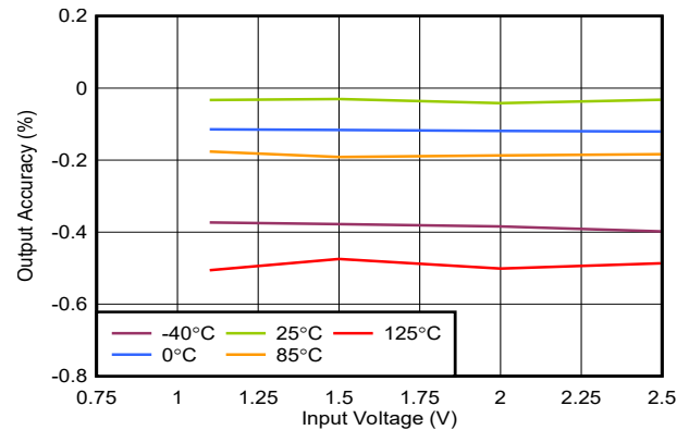
Figure 5-20. Output Voltage Accuracy vs V_{IN}
