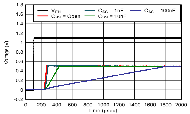
Figure 5-14. Start-Up for C_{SS}
