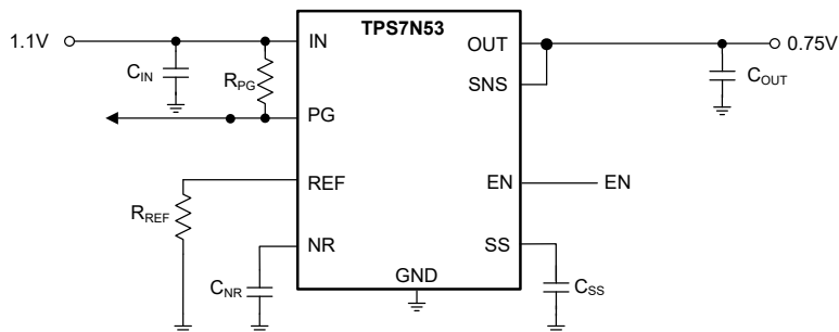
Figure 7-5. Typical Circuit
