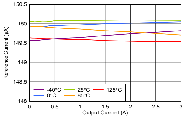
Figure 5-19. Reference Current Accuracy vs I_{OUT}
