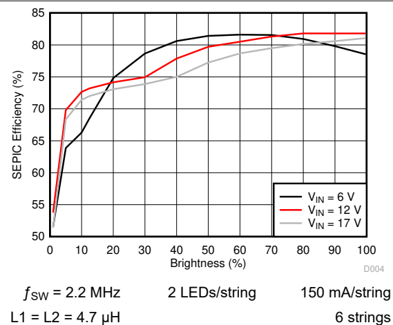
Figure 6-5. SEPIC Efficiency
