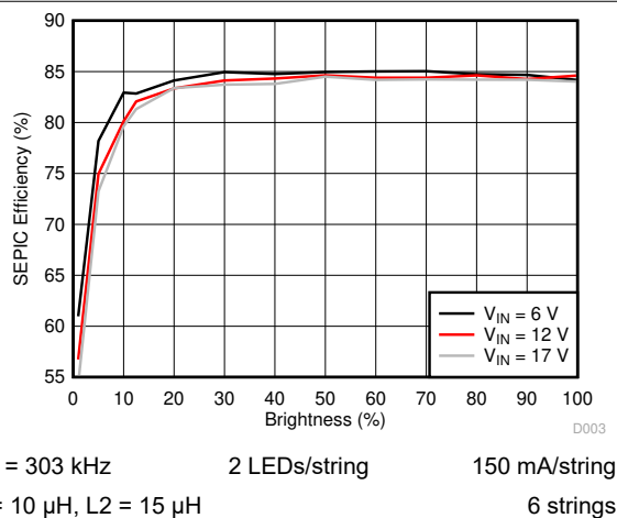
Figure 6-4. SEPIC Efficiency
