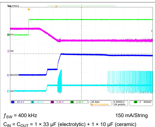
Figure 8-4. Typical Start-Up
