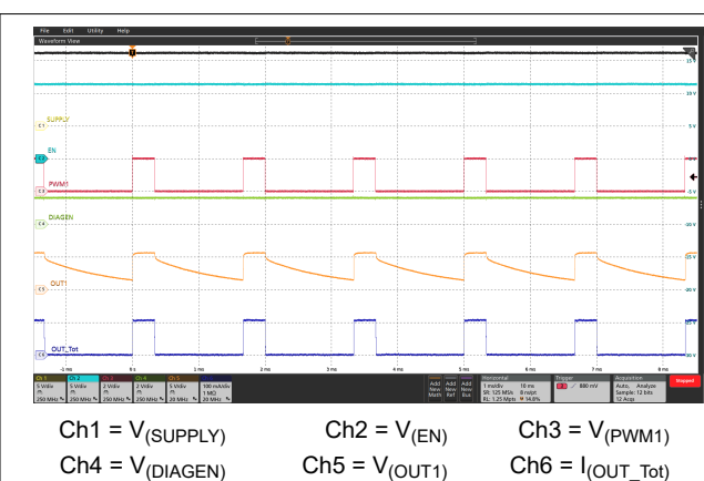
Figure 8-6. PWM Dimming 20% Dutycycle at 600 Hz
