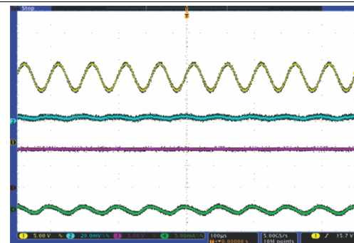
CH1: V_{(SUPPLY)} CH2: V_{(REF)} CH3: V_{(IOUT8)} CH4: I_{(IOUT8)} I_{(IOUTx)} = 35 \text{ mA}
