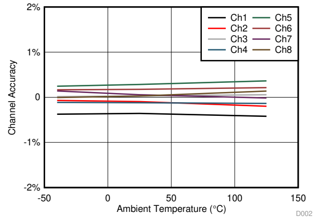
Figure 2. I_{(IOUTX)} Accuracy vs Ambient Temperature
