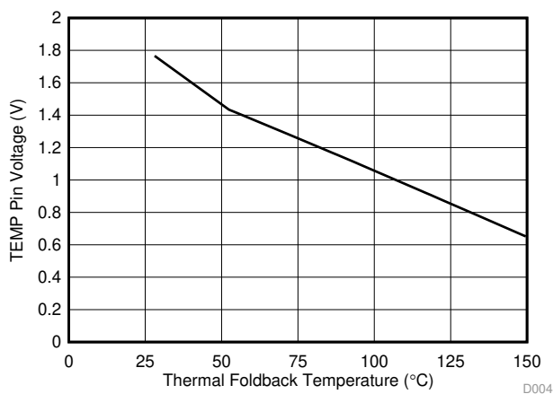
Figure 36. TEMP Pin Voltage vs Thermal Foldback Temperature
