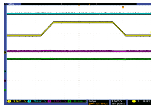
CH1: V_{(SUPPLY)} CH2: V_{(REF)} CH3: V_{(FAULT)} I_{(OUTx)} = 35 mA
