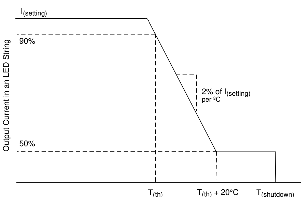
Figure 35. Thermal Foldback
