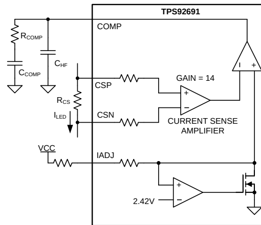
Figure 31. Proportional-Integral Compensation
