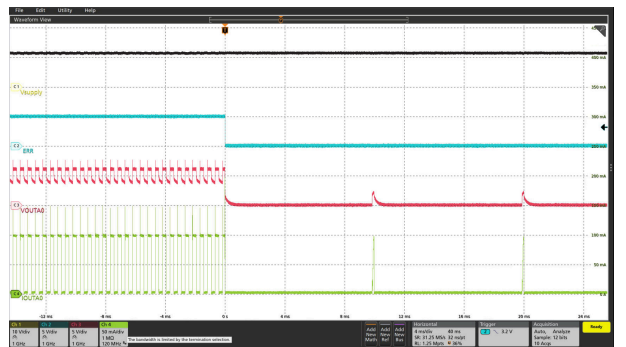
Figure 5-30. LED Short-Circuit Detection in Fail-Safe Mode
