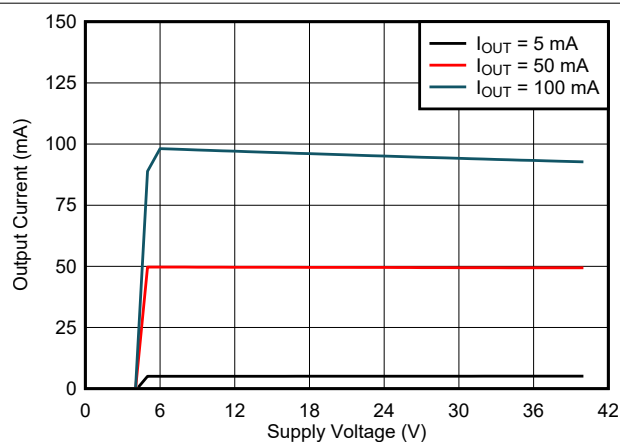
Figure 5-5. Output Current vs Supply Voltage
