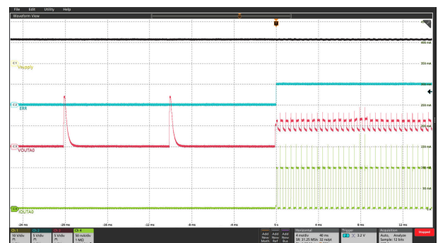
Figure 5-27. Single-LED Short-Circuit Detection in Normal Mode
