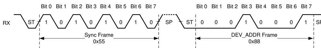
Figure 6-15. Synchronization Byte
