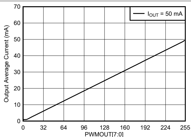
Figure 5-6. Average Current vs PWMOUT[7:0]
