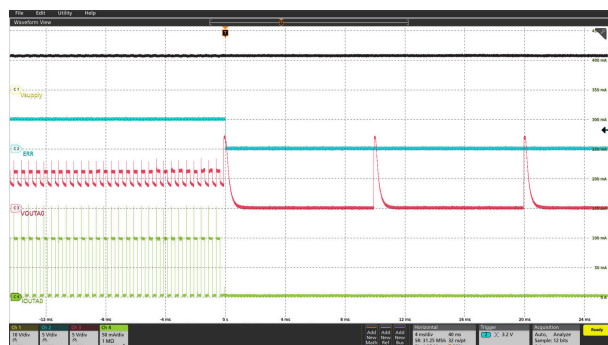
Figure 5-26. LED Short-Circuit Detection in Normal Mode
