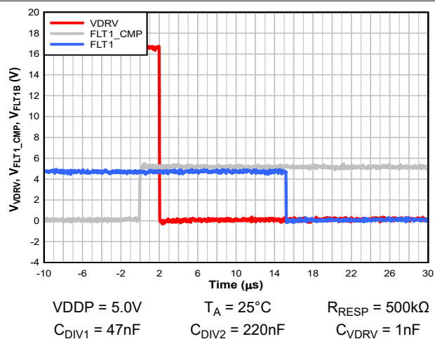
Figure 6-12. t_{\text{PD\_CMP\_VDRV\_DIS}} , t_{\text{FLT\_LATENCY}}
