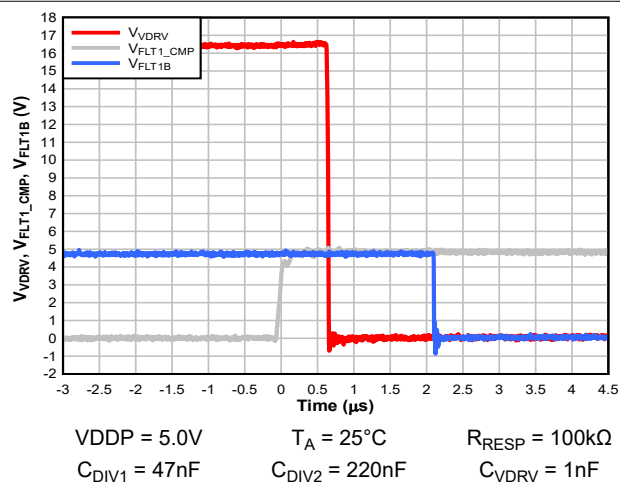
Figure 6-11. t_{\text{PD\_CMP\_VDRV\_DIS}} , t_{\text{FLT\_LATENCY}}
