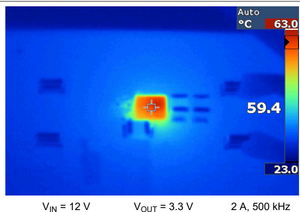
Figure 8-14. EVM Thermal Performance
