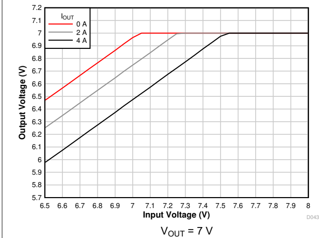
Figure 7-11. Voltage Dropout
