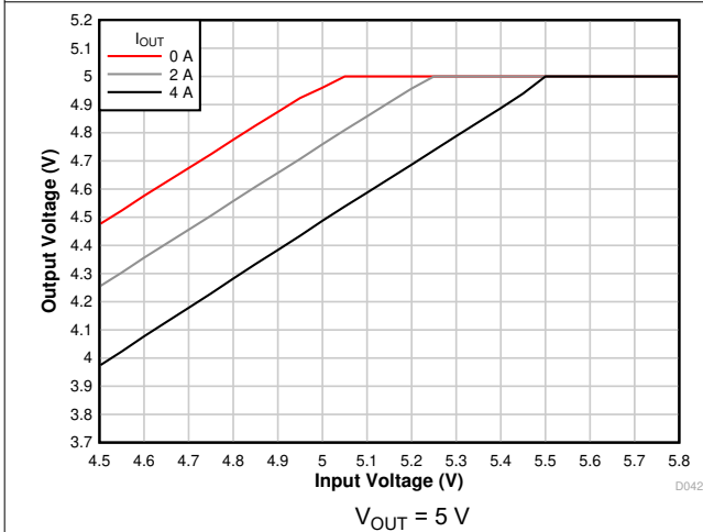
Figure 7-9. Voltage Dropout
