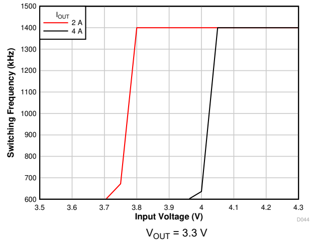
Figure 7-8. Frequency Foldback
