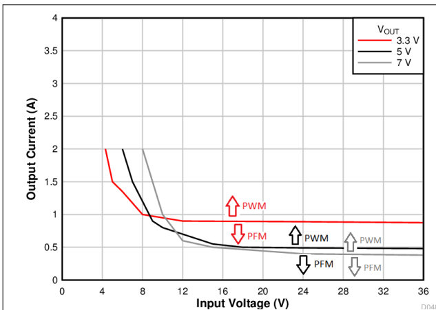
Figure 7-14. PFM/PWM Thresholds (3.3 V, 5 V, and 7 V)
