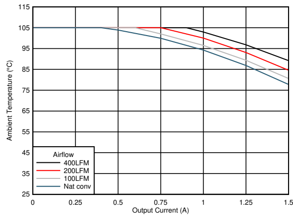
Figure 7-20. Safe Operating Area ( V_{OUT} = 3.3\text{ V} )
