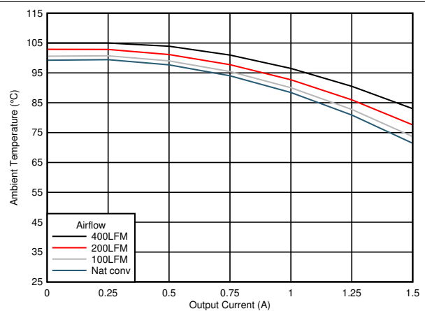
Figure 7-22. Safe Operating Area ( V_{OUT} = 5.0\text{ V} )
