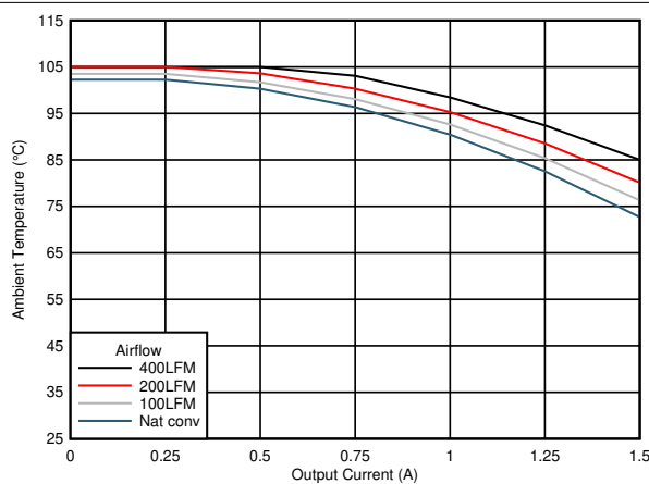
Figure 7-23. Safe Operating Area ( V_{OUT} = 12\text{ V} )
