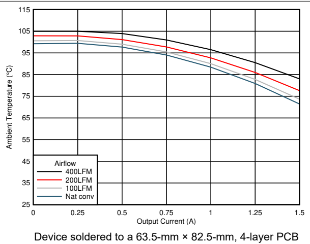
Figure 7-24. Safe Operating Area (V OUT = 15 V)
