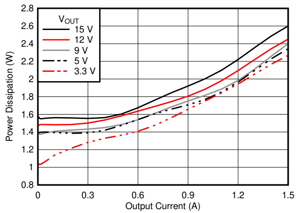
Figure 7-20. Power Dissipation
