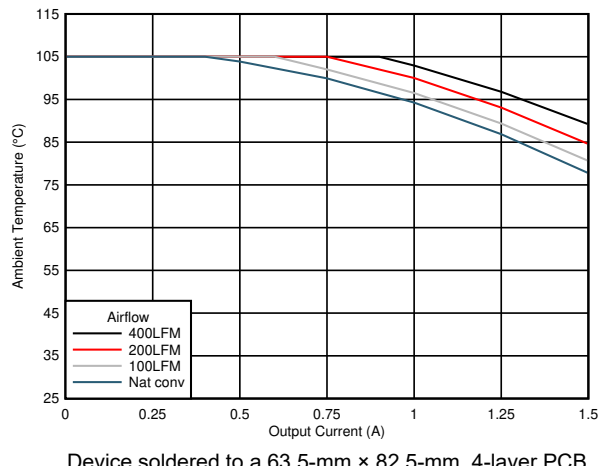
Figure 7-22. Safe Operating Area (V OUT = 5.0 V)
