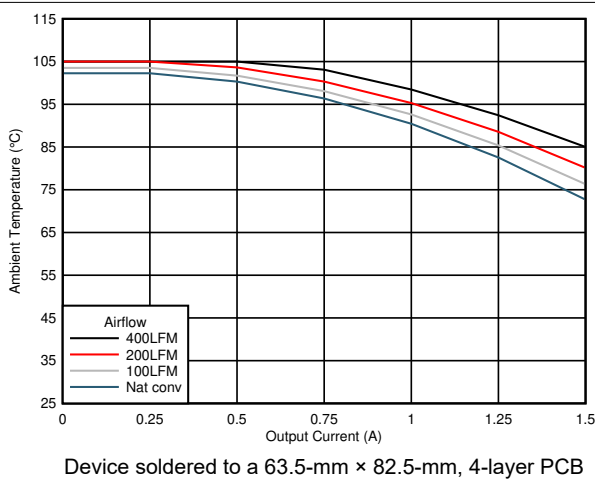
Figure 7-23. Safe Operating Area (V OUT = 12 V)
