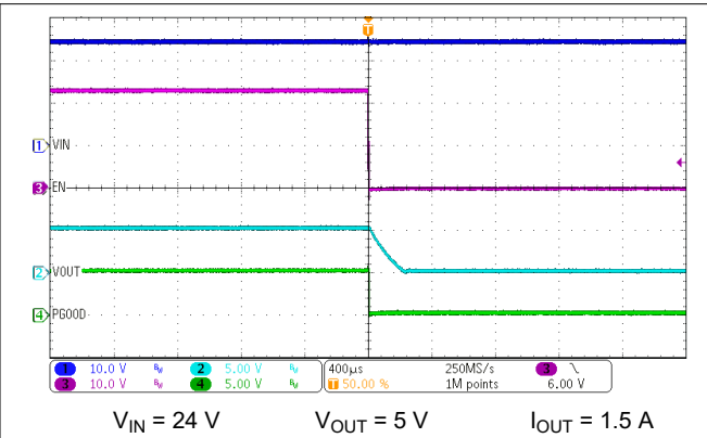
Figure 9-3. Enable Shutdown Waveforms
