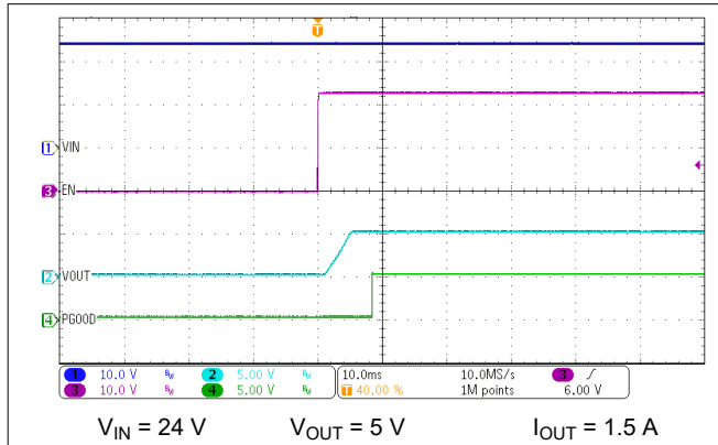
Figure 9-2. Start-up Waveforms
